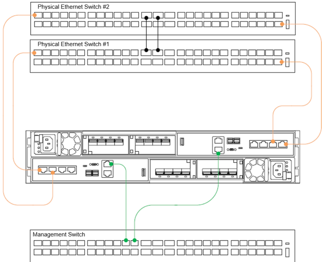
Figure 35. PowerStore T model appliance minimum cabling
