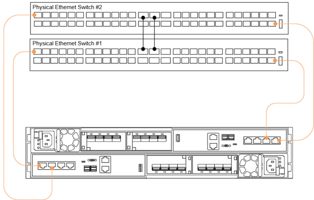
Figure 39. PowerStore X model minimum cabling
