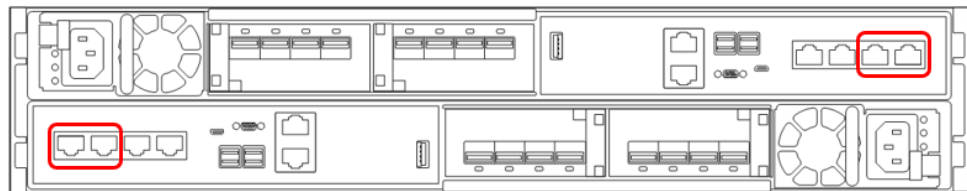
Figure 36. PowerStore T model system bonds
