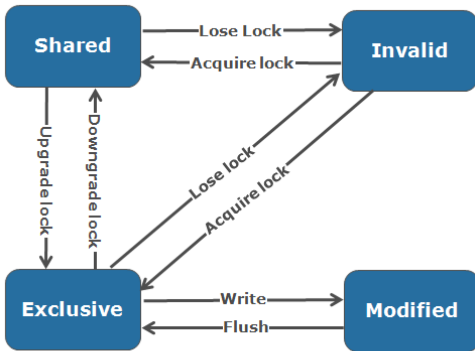
Figure 2: OneFS Cache Coherency State Diagram
