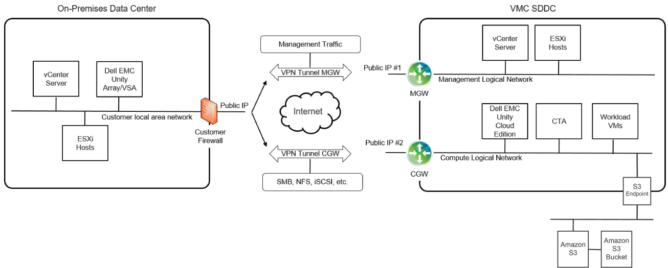
Figure 5 Solution networking overview diagram
