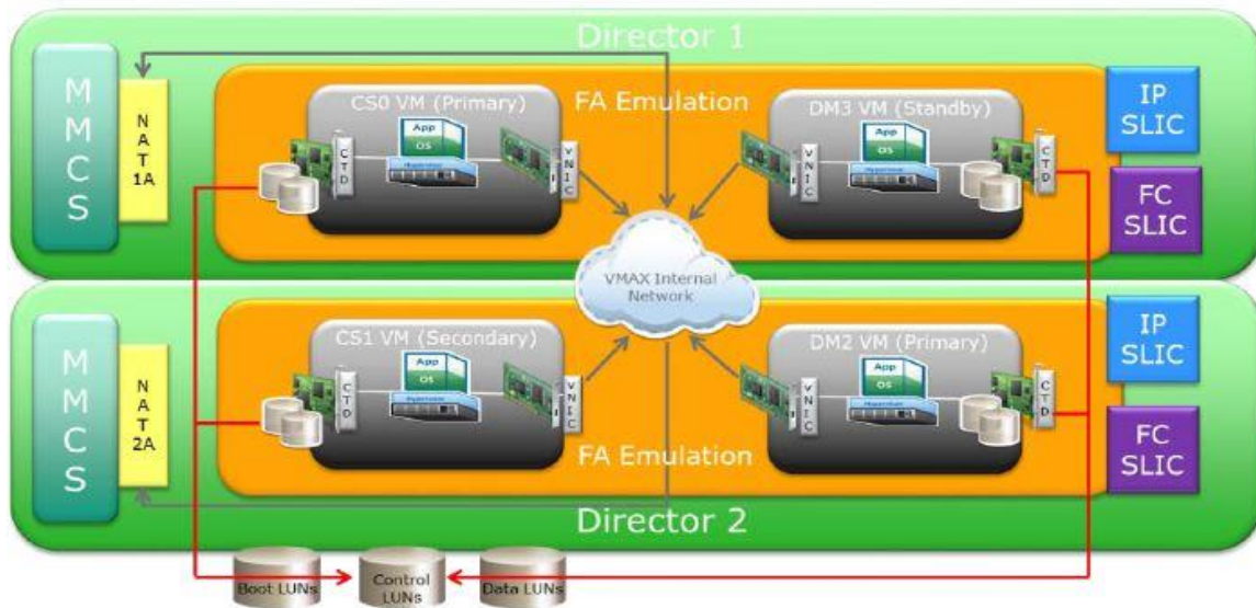
Figure 1 eNAS architecture
