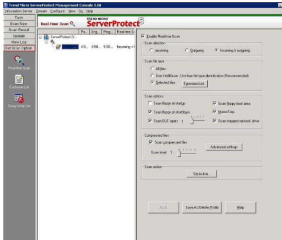
Figure 1 Trend Micro ServerProtect Real-time Scan options window
