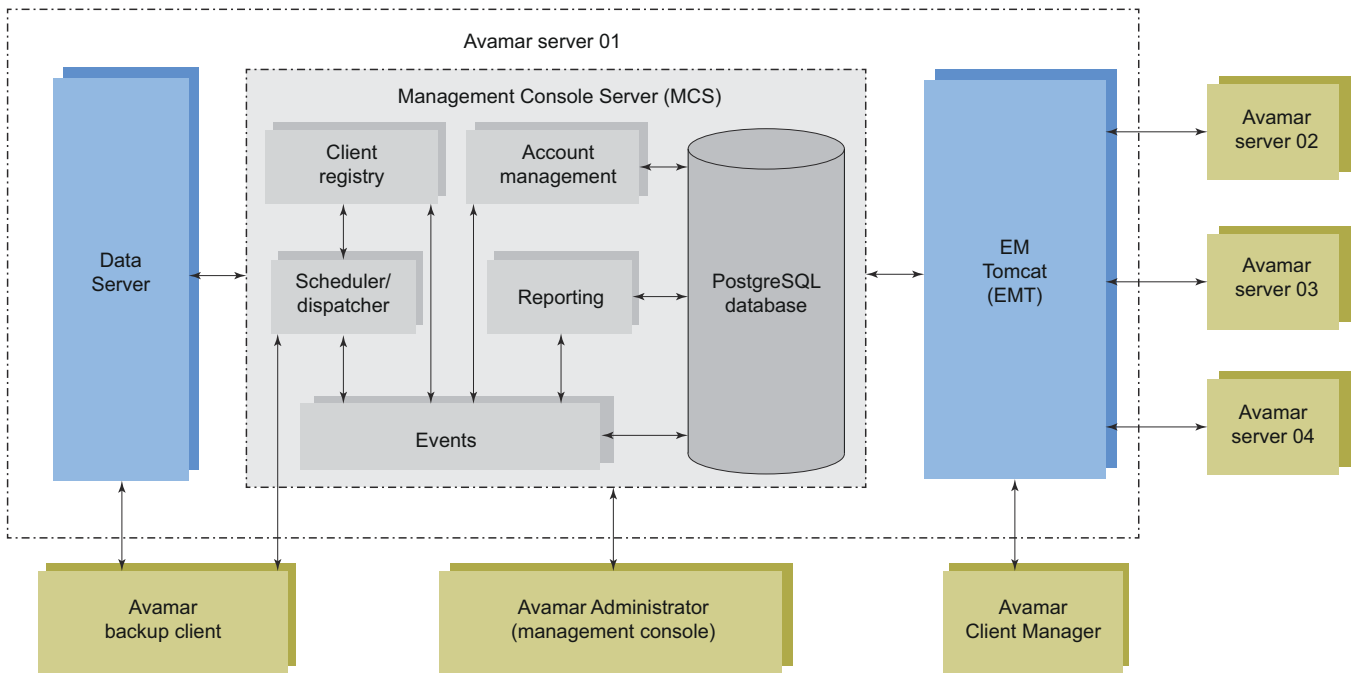
Figure 2 Avamar server functional block diagram
