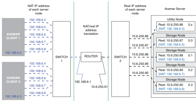
Figure 15 Multi-node server configuration with NAT
