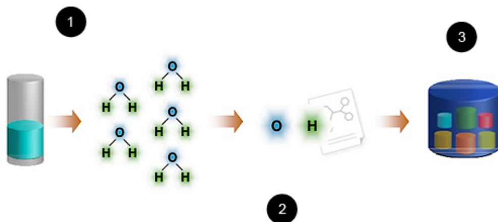
Figure 4 Data deduplication
