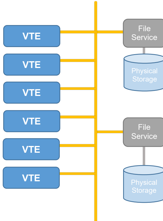
Figure 2. DLm8500 Architecture
