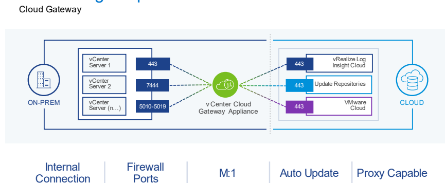
Figure 17. Network considerations when deploying vCenter Cloud Gateway Appliance
