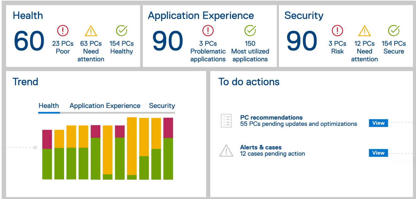
Simulated dashboard
