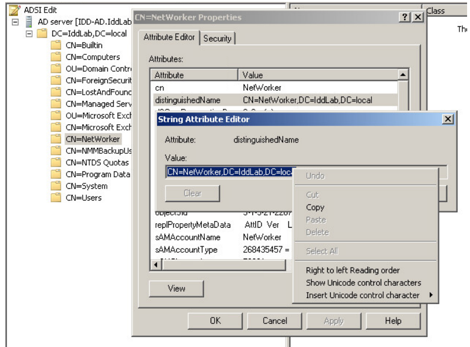
Figure 83 Copying the group DN
