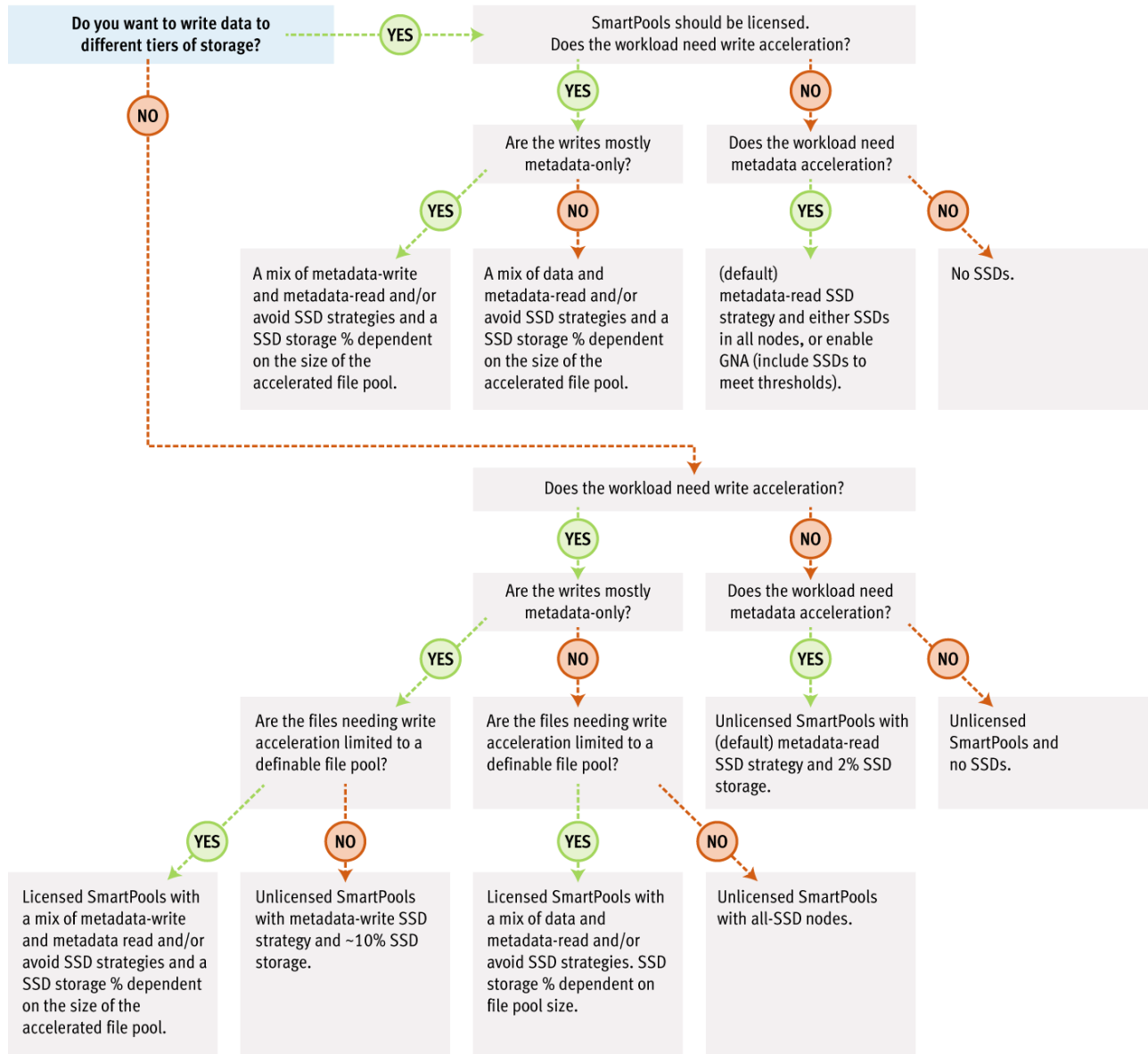
Figure 7. SSD usage decision tree
