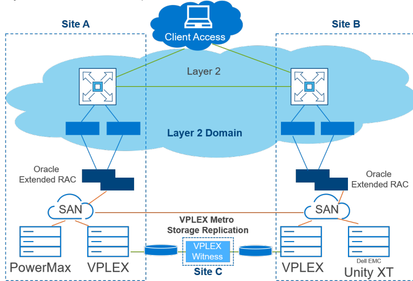
Figure 1. Solution Architecture: FC=Orange, Ethernet=Blue and IP=Green
