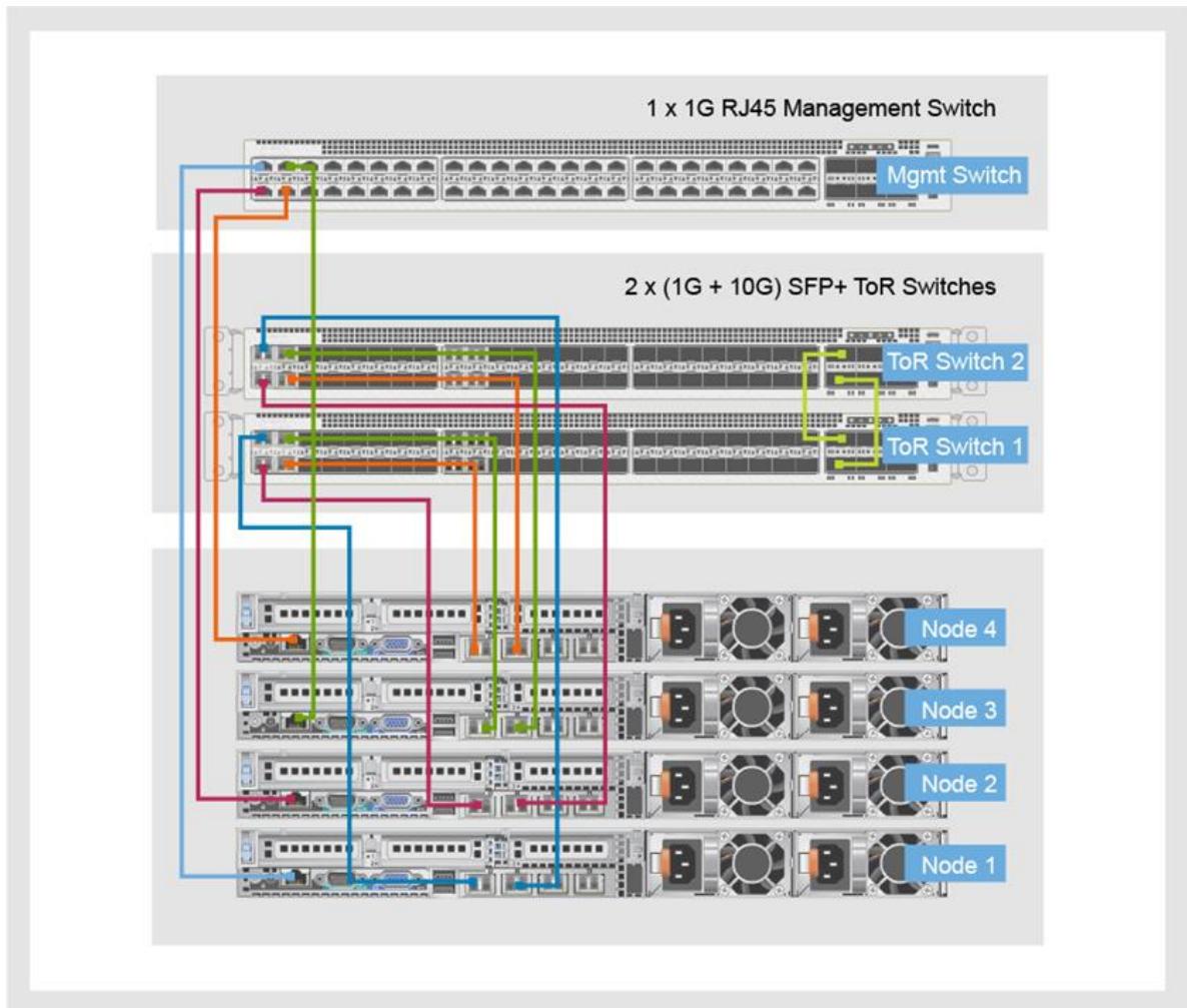
Figure 20. Typical VxRail physical network connectivity for 10 GbE configurations
