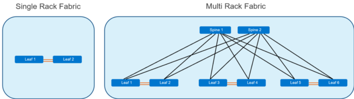
Figure 22. SmartFabric enabled multi-rack network expansion
