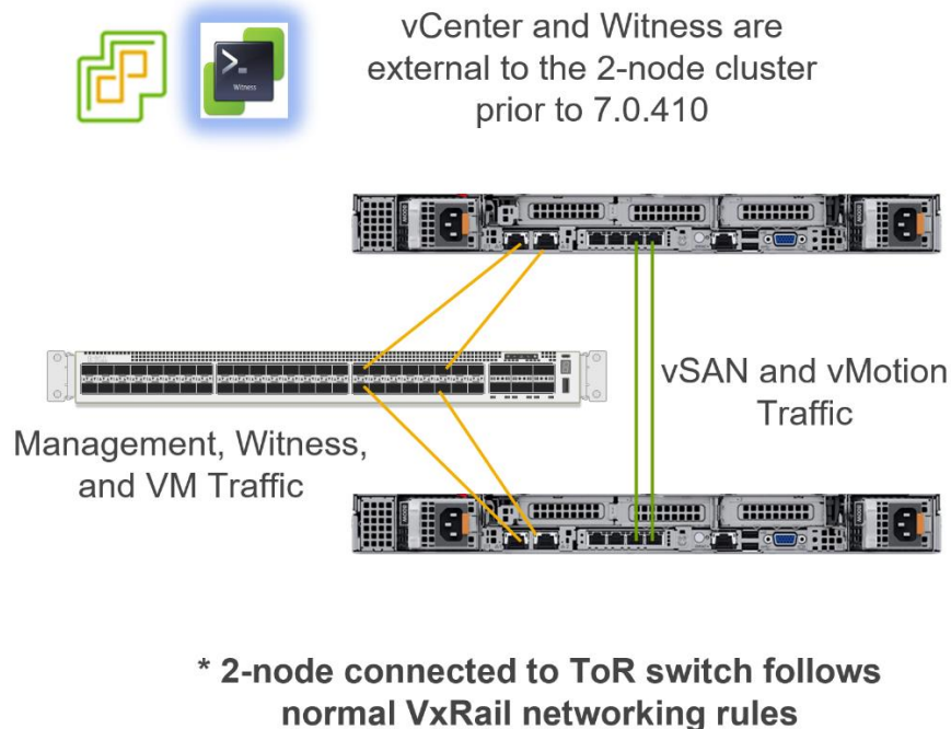
Figure 27. Network configuration for a 2-node vSAN cluster deployed with direct-connect option
