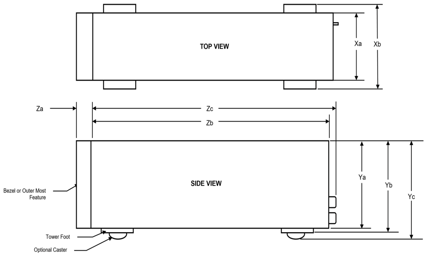
Figure 16. Chassis dimensions
