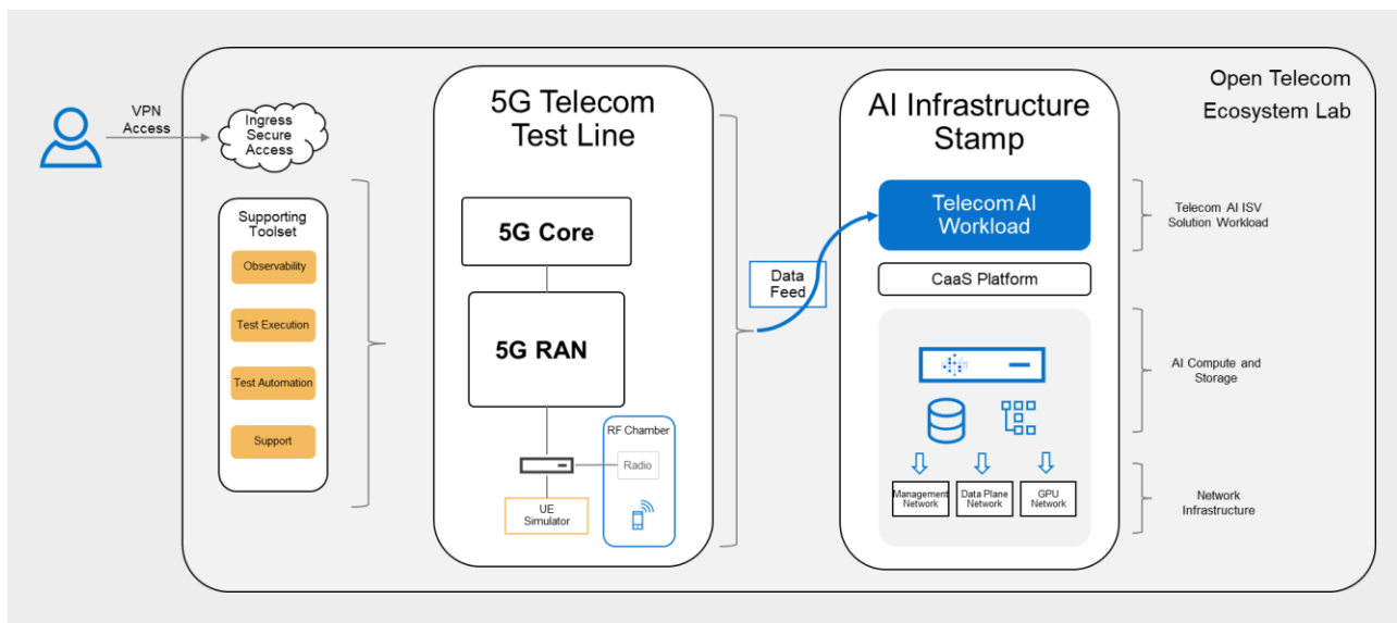
Dell Telecom AI Solution Certification Test Line in OTEL
