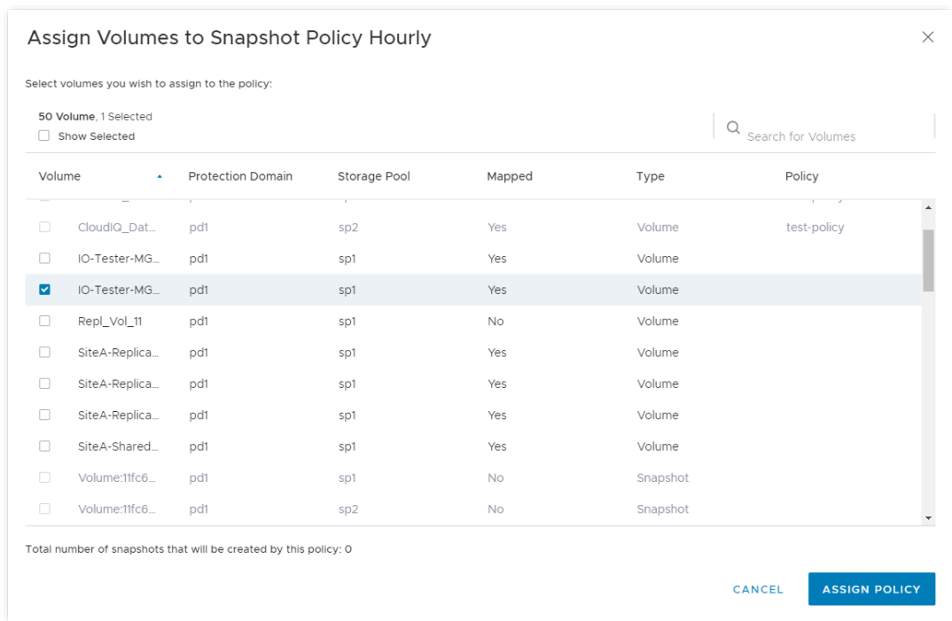
Figure 13. Assign Volumes to Snapshot Policy
