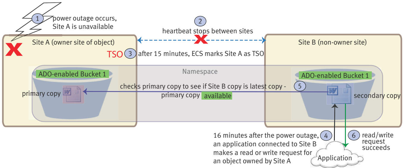
Figure 15 Read/write request succeeds during TSO when ADO-enabled data is accessed from non-owner site and owner site is unavailable
