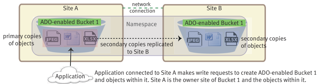
Figure 16 Object ownership example for a write during a TSO in a two-site federation
