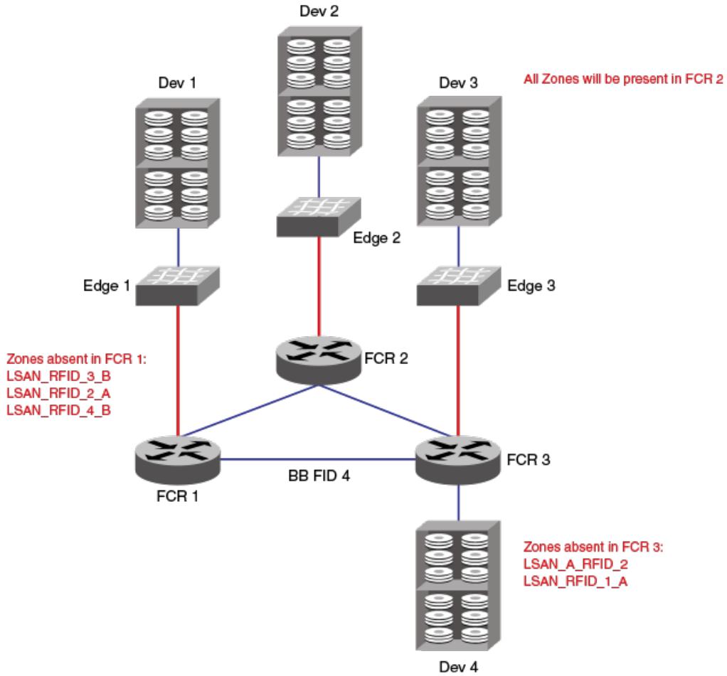
FIGURE 81 Sample location-embedded LSAN zones environment
