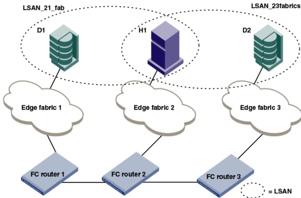
FIGURE 78 Example of setting up Enforce LSAN tag
