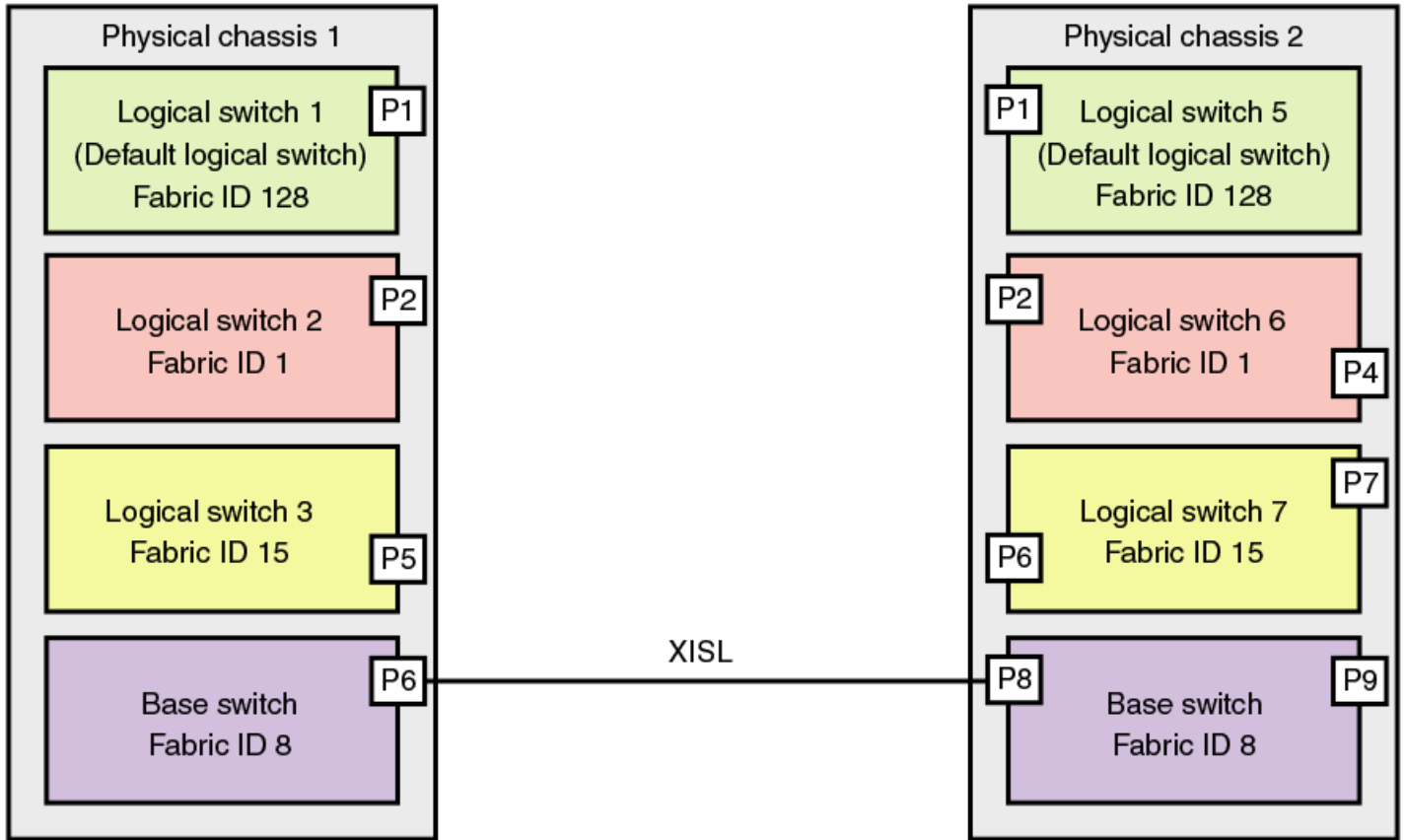
FIGURE 26 Base switches connected by an XISL
