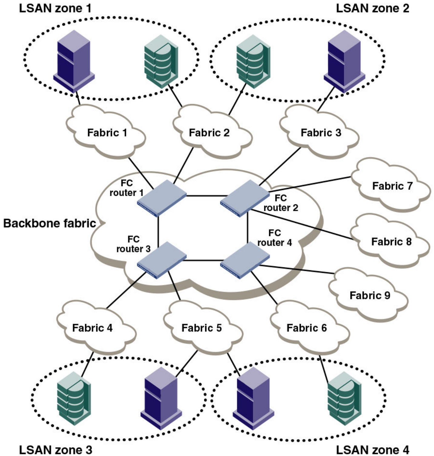
FIGURE 80 LSAN zone binding
