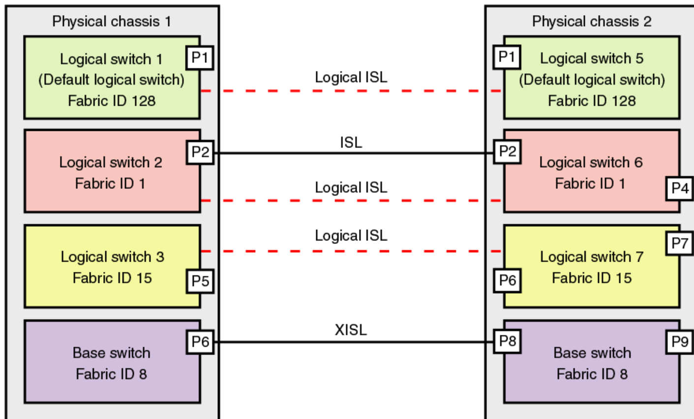
FIGURE 28 Logical fabric using ISLs and XISLs
