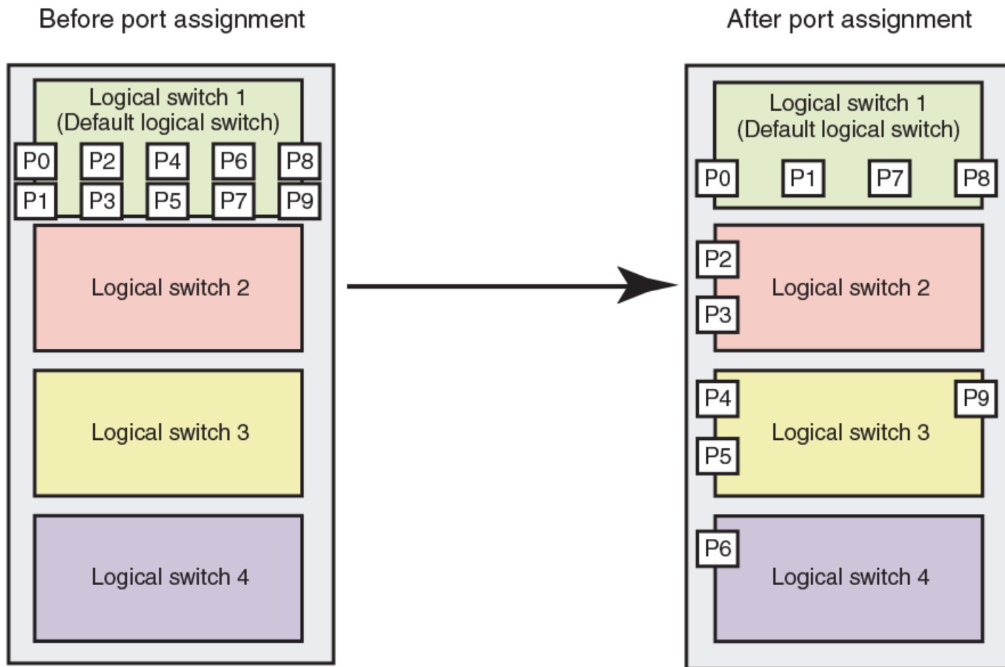
FIGURE 21 Assigning ports to logical switches
