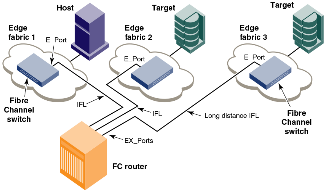
FIGURE 71 A metaSAN with inter-fabric links
