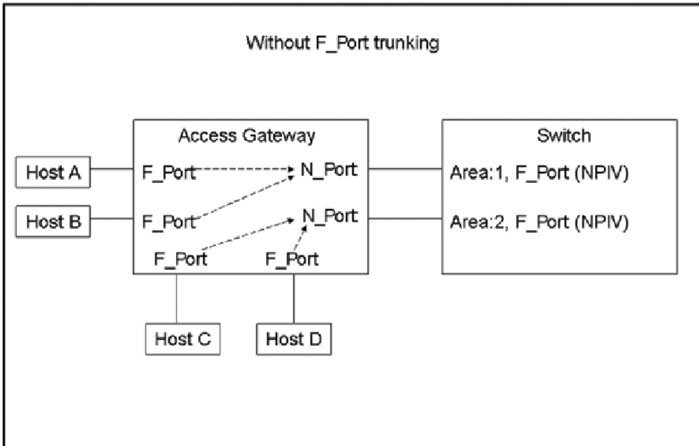
FIGURE 69 Switch in Access Gateway mode without F_Port masterless trunking
