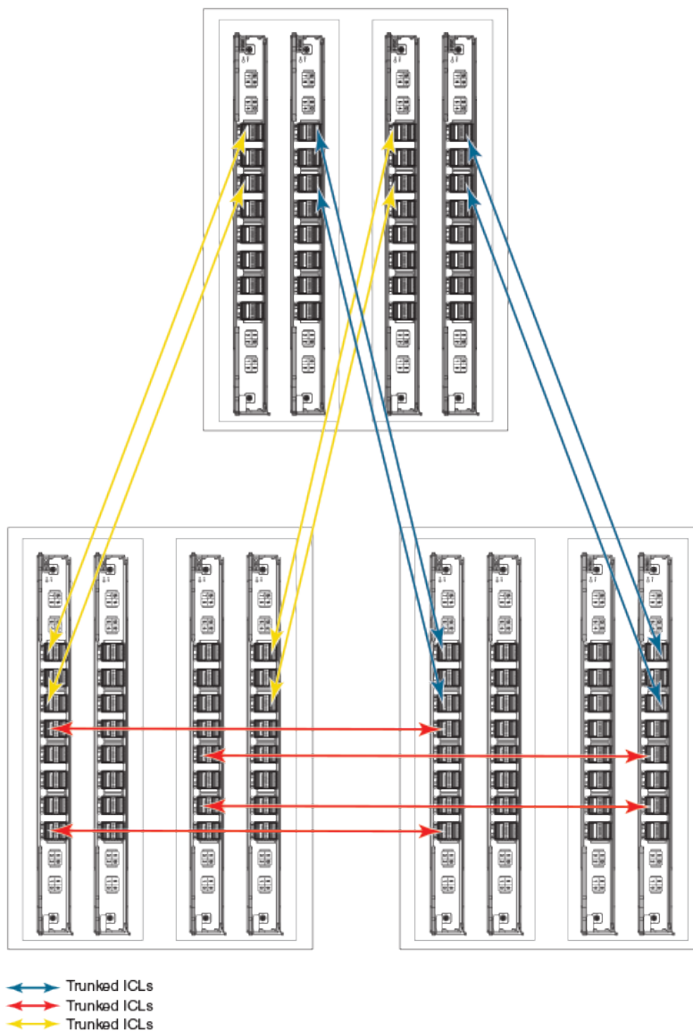
FIGURE 65 Three Brocade X6-8 chassis in full mesh triangular ICL topology
