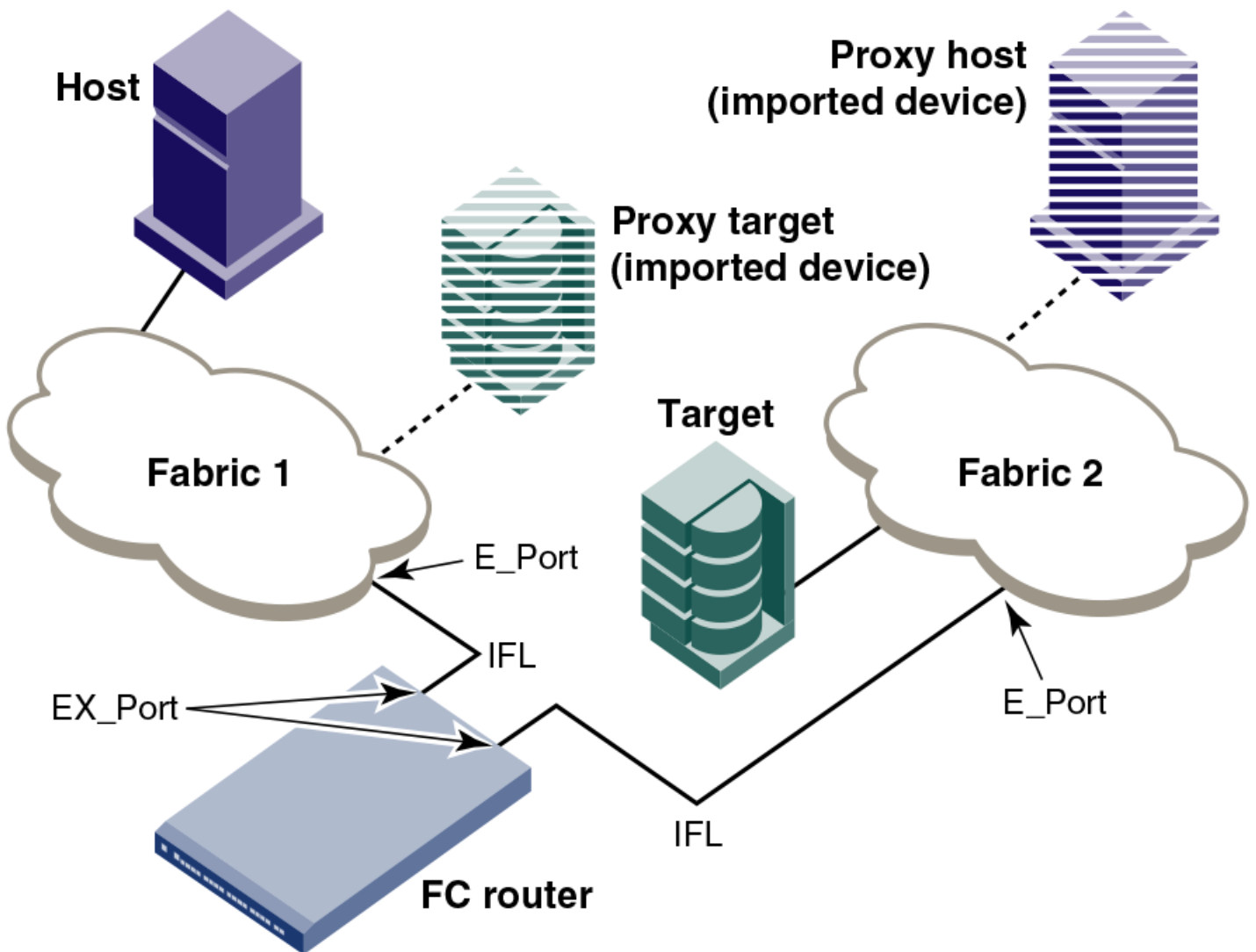
FIGURE 74 MetaSAN with imported devices
