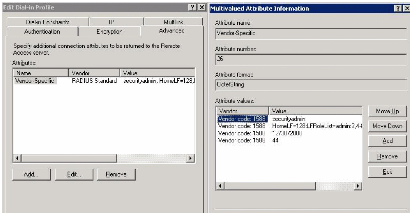
FIGURE 10 Windows 2012 VSA configuration
