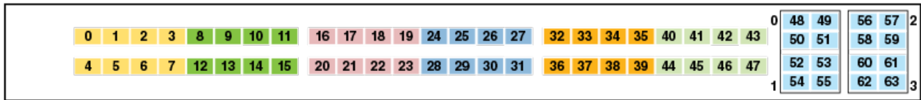
FIGURE 68 Port group configuration for the Brocade G620
