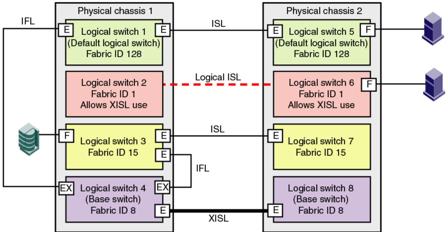
FIGURE 82 EX_Ports in a base switch
