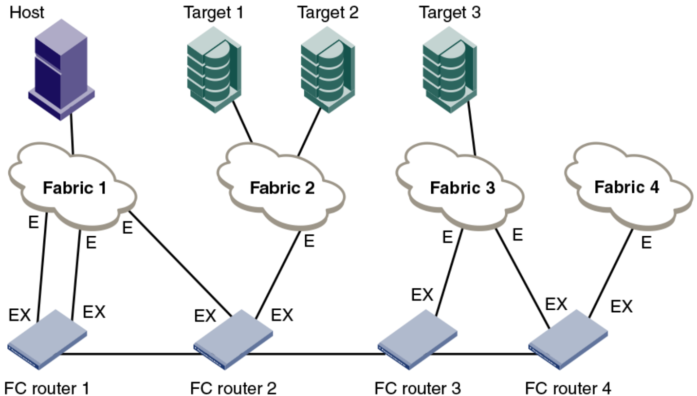
FIGURE 75 Sample topology (physical topology)
