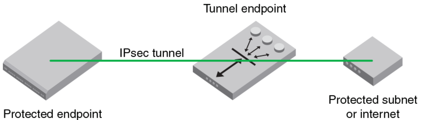
FIGURE 17 Endpoint-to-gateway tunnel configuration
