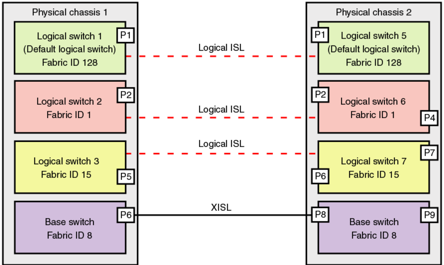
FIGURE 27 Logical ISLs connecting logical switches
