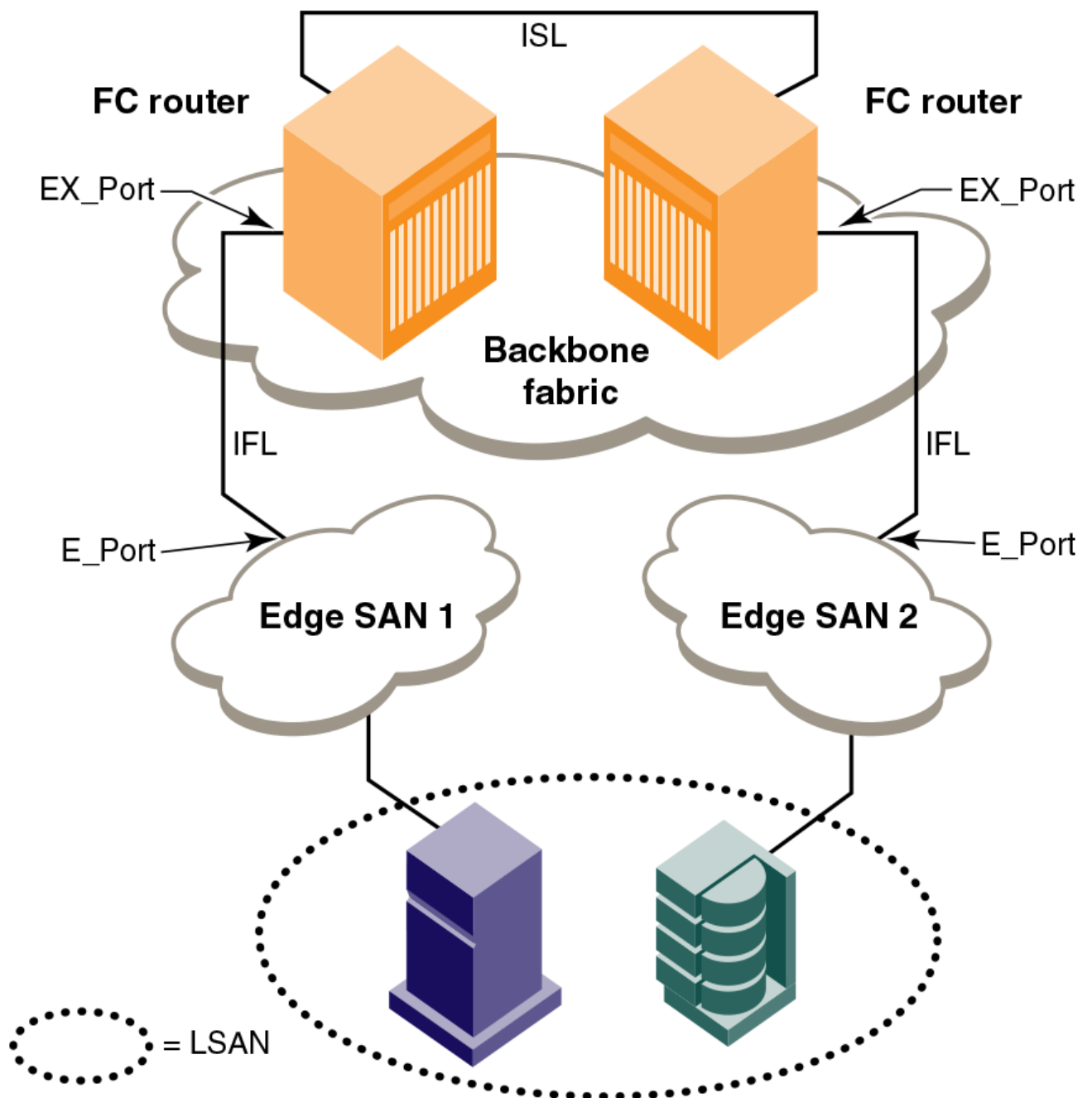
FIGURE 73 Edge SANs connected through a backbone fabric
