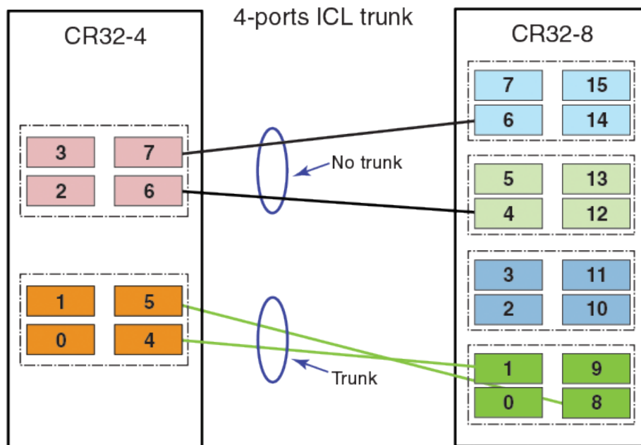
FIGURE 62 ICL trunking for X6 core routing blades
