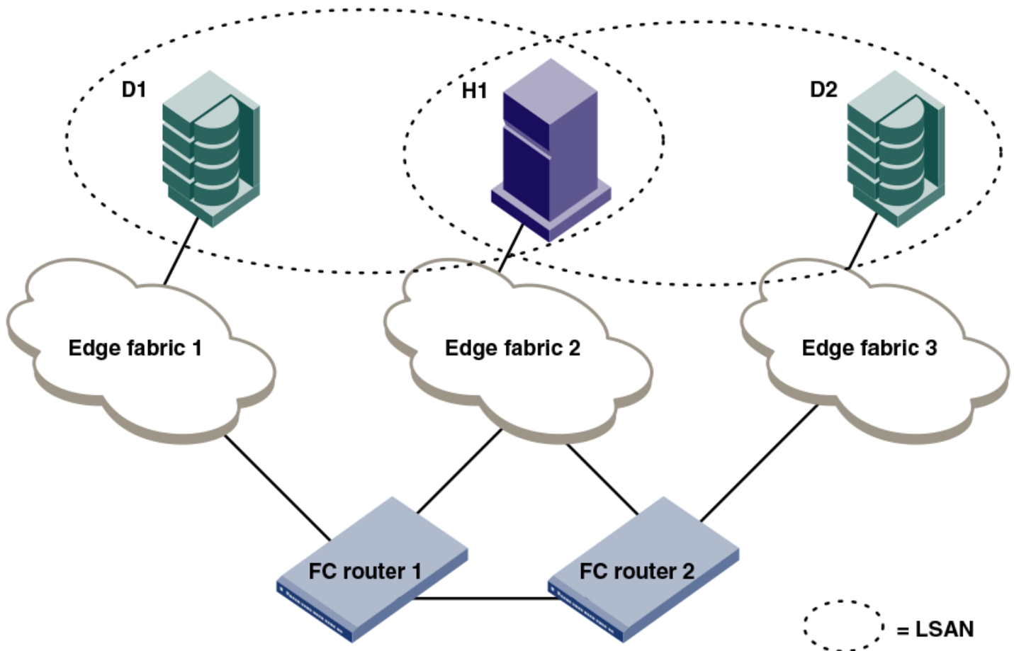
FIGURE 79 Example of setting up Speed LSAN tag
