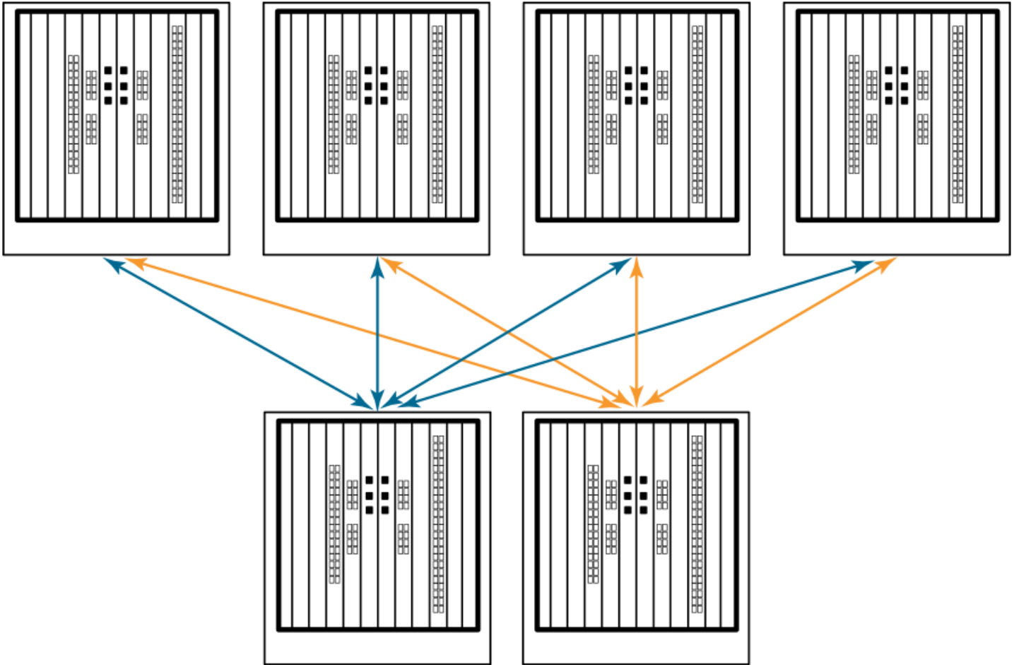
FIGURE 67 Illustration of ICL core-edge topology using Brocade chassis platforms
