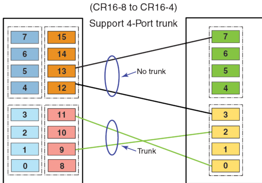
FIGURE 60 ICL trunking boundaries
