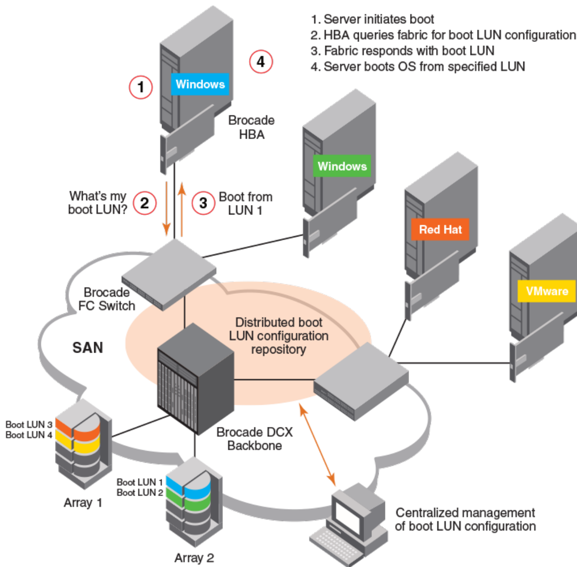
FIGURE 35 Boot LUN zoning
