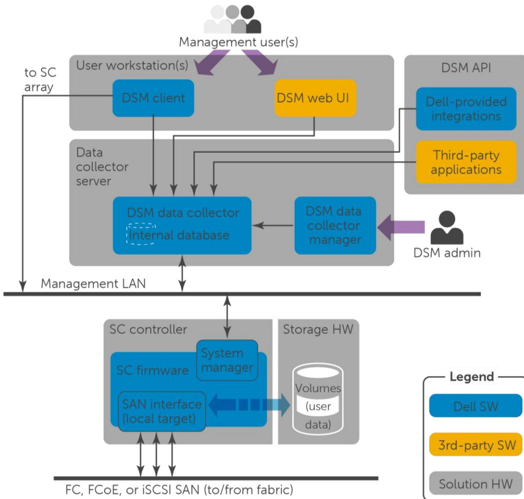
Figure 1 Functional block diagram of the Dell SAN components
