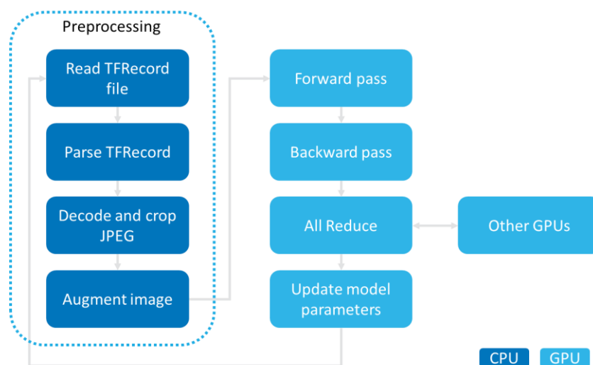
Figure 11: TensorFlow Training pipeline
