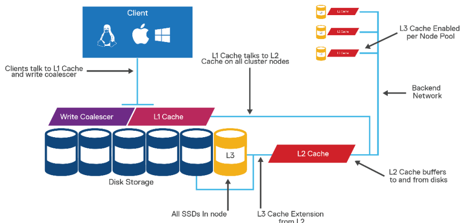
Figure 6: OneFS Caching Architecture
