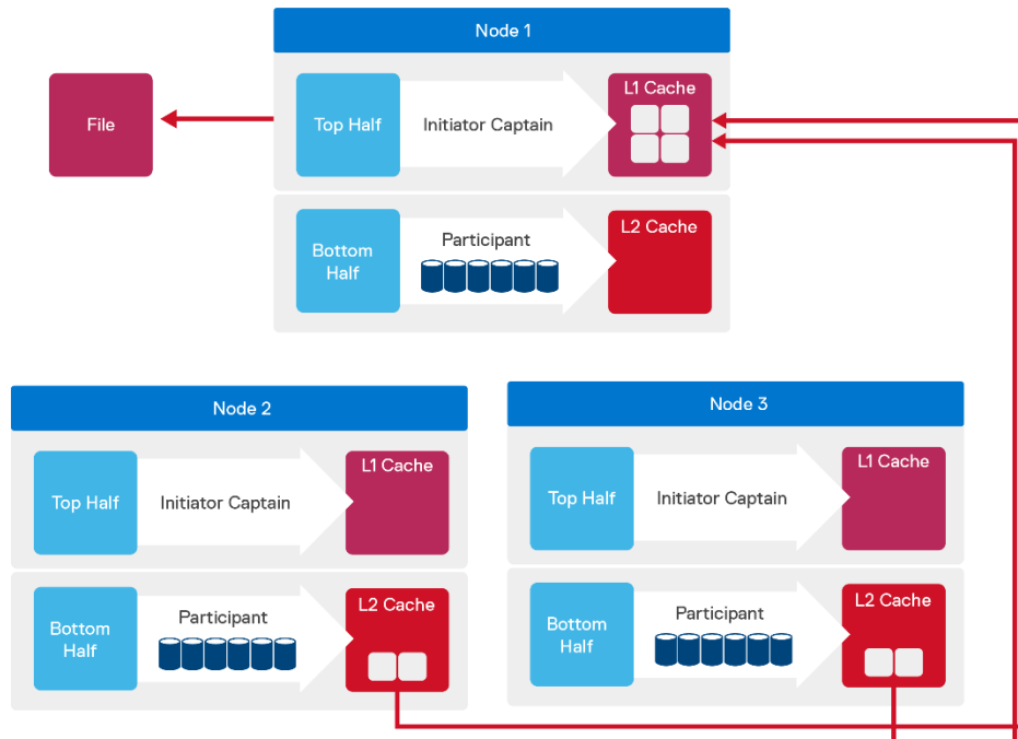
Figure 7: A File Read Operation on a 3-node Isilon Cluster
