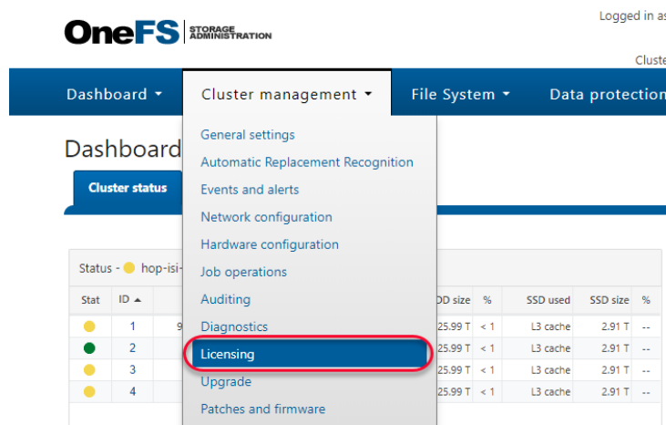
Figure 34. Verifying licenses
