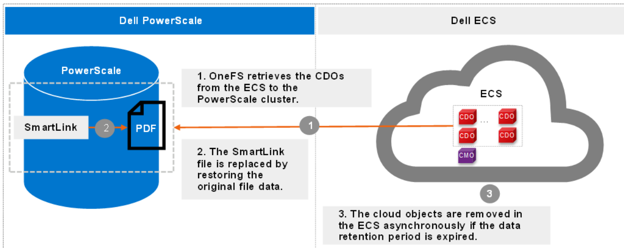
Figure 4. Recall workflow
