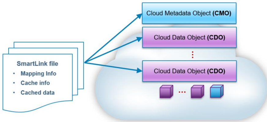
Figure 2. SmartLink file
