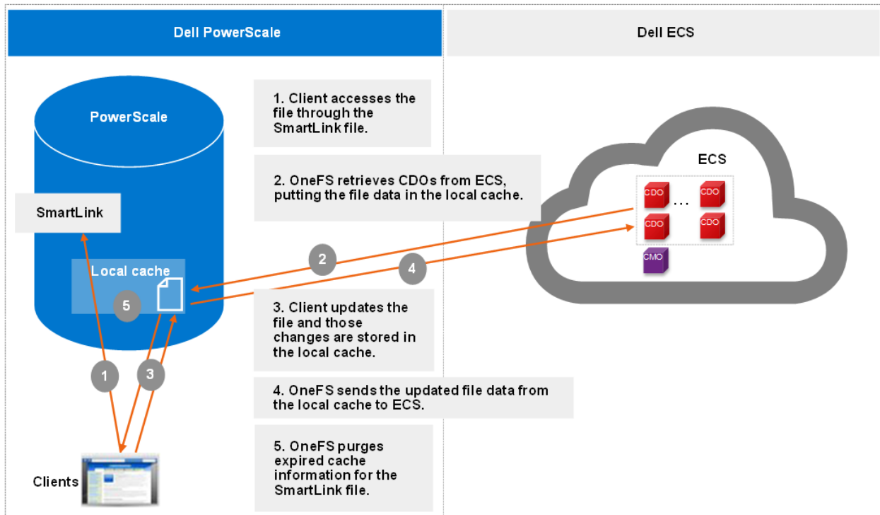
Figure 6. Update workflow
