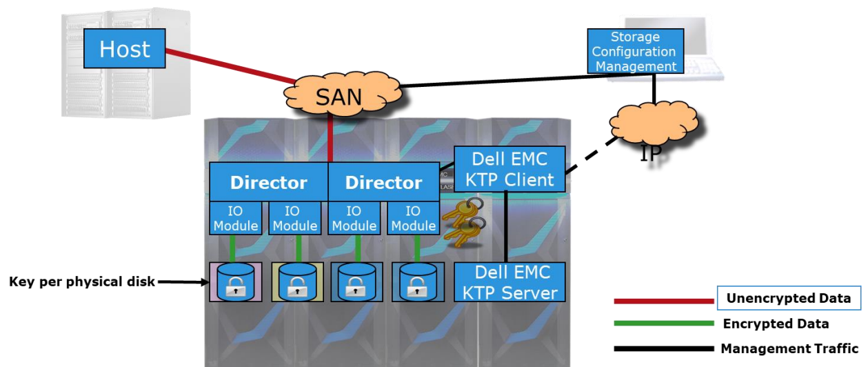
Figure 1 Embedded key manager architecture
