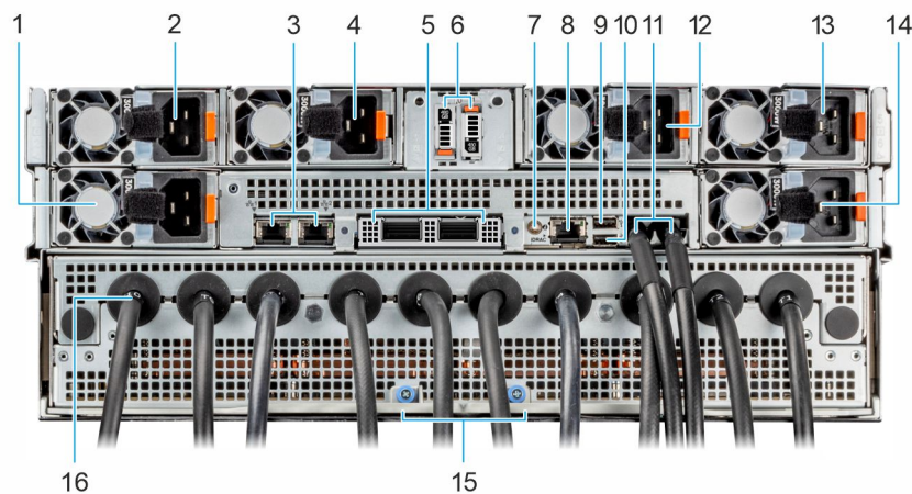
Figure 3. Rear view of the system
