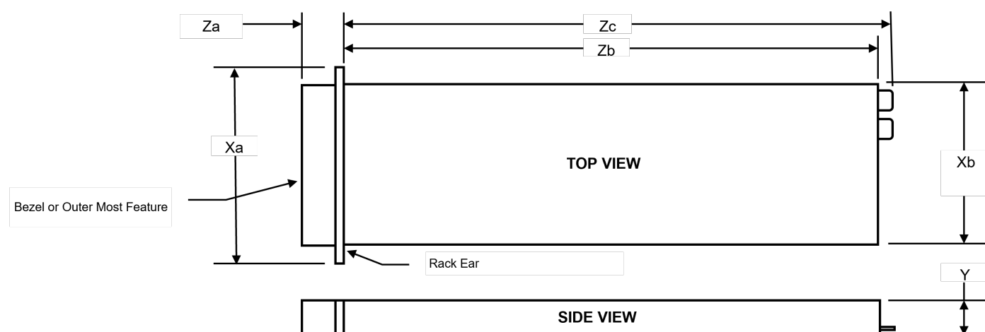
Figure 17. Chassis dimensions
