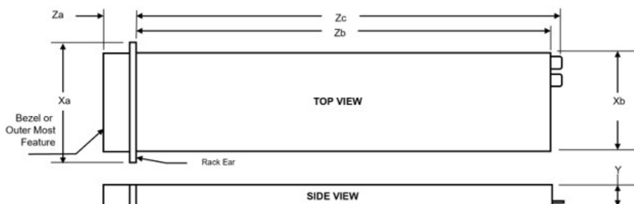
Figure 24. Chassis dimensions
