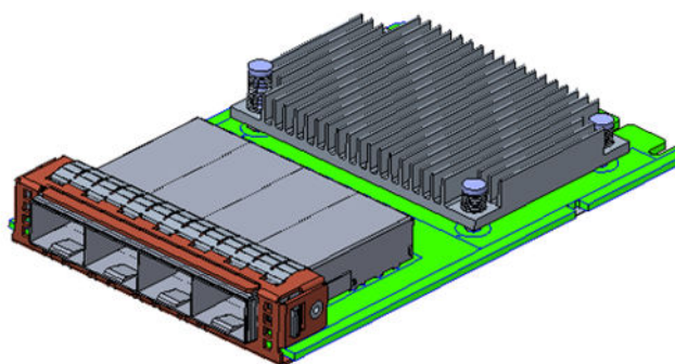
Figure 11. OCP 3.0 Small Card Form Factor (LS)
