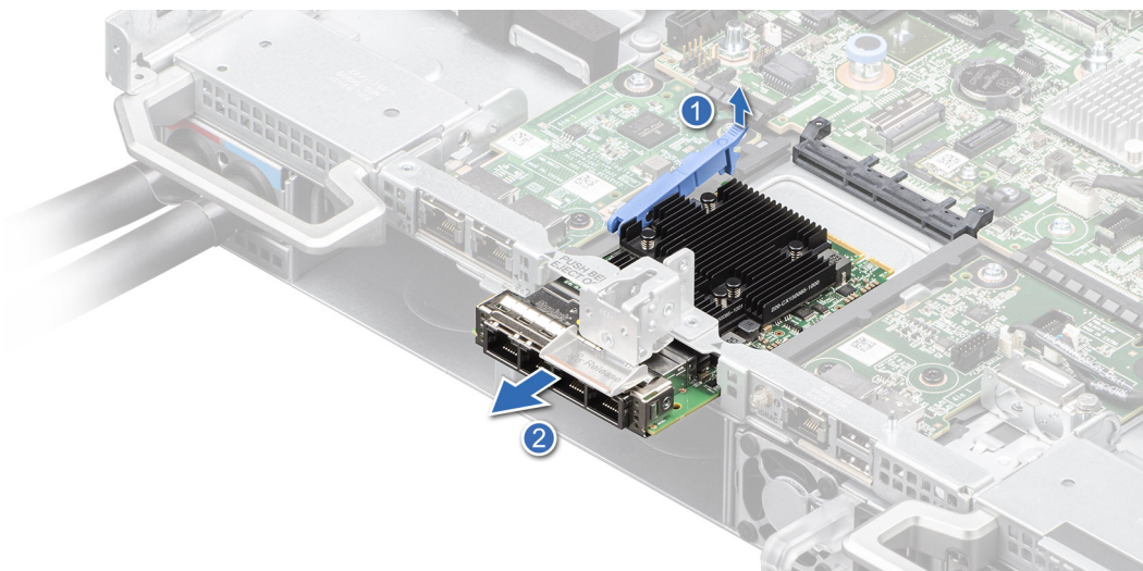
Figure 13. Removing the OCP Card in XE9640
