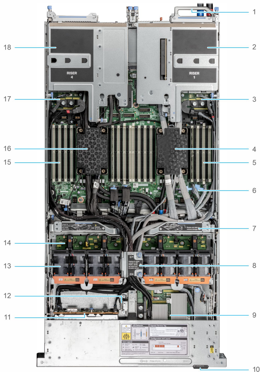
Figure 6. Top layer of XE9640 with NVIDIA GPUs - inside the system
