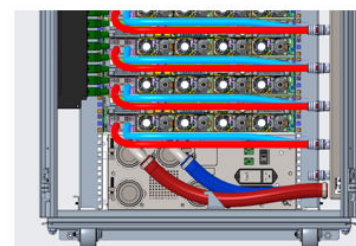
Detail of manifold and in-rack CDU. End of row CDU (CHx750) likely to be used for large deployments.
