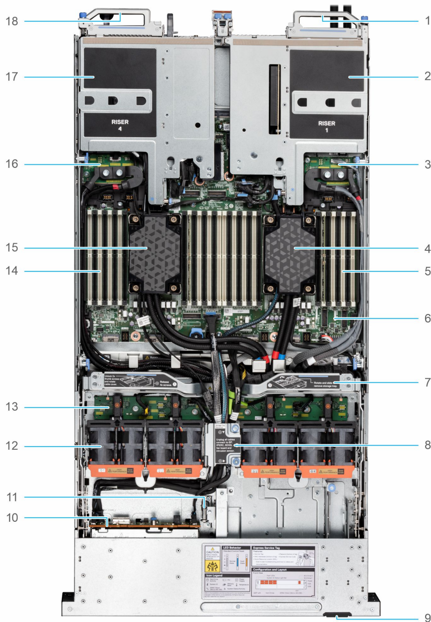
Figure 4. Top layer of the XE9640 system with Intel GPUs - inside the system
