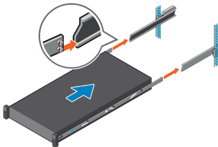
Figure 22. Install system into the extended rails
