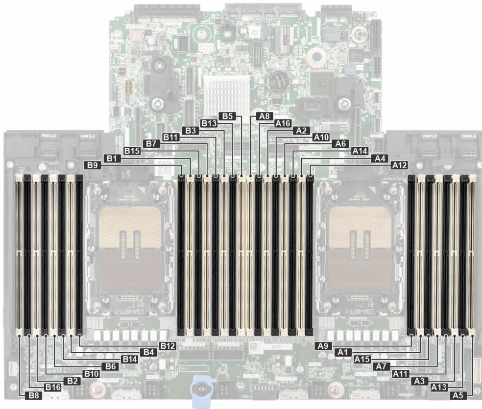
Figure 9. Memory channels
