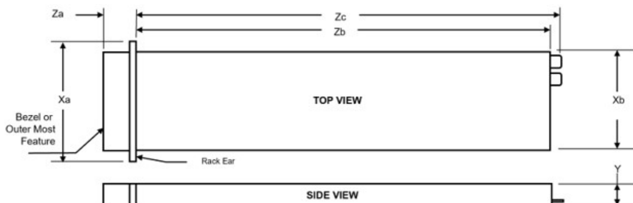
Figure 21. Chassis dimensions
