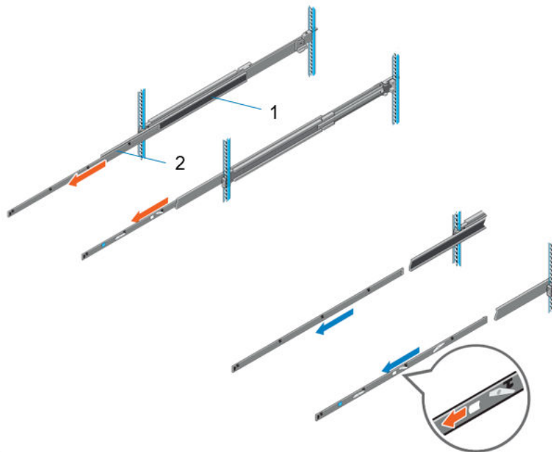
Figure 20. Pull out the intermediate rail
