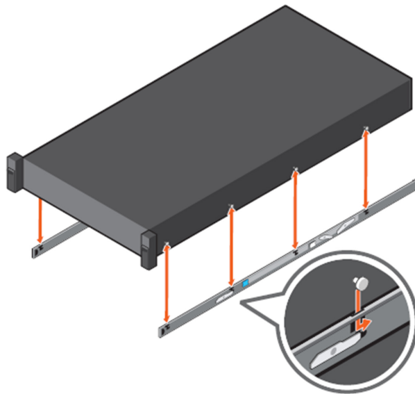
Figure 21. Attach the inner rails to the system
