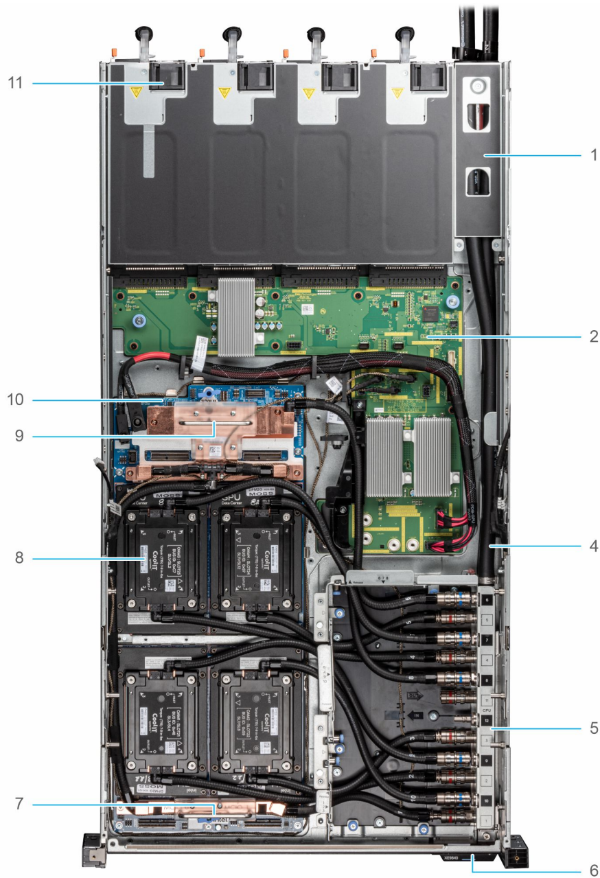
Figure 5. Bottom layer of the XE9640 system with Intel GPUs - inside the system
