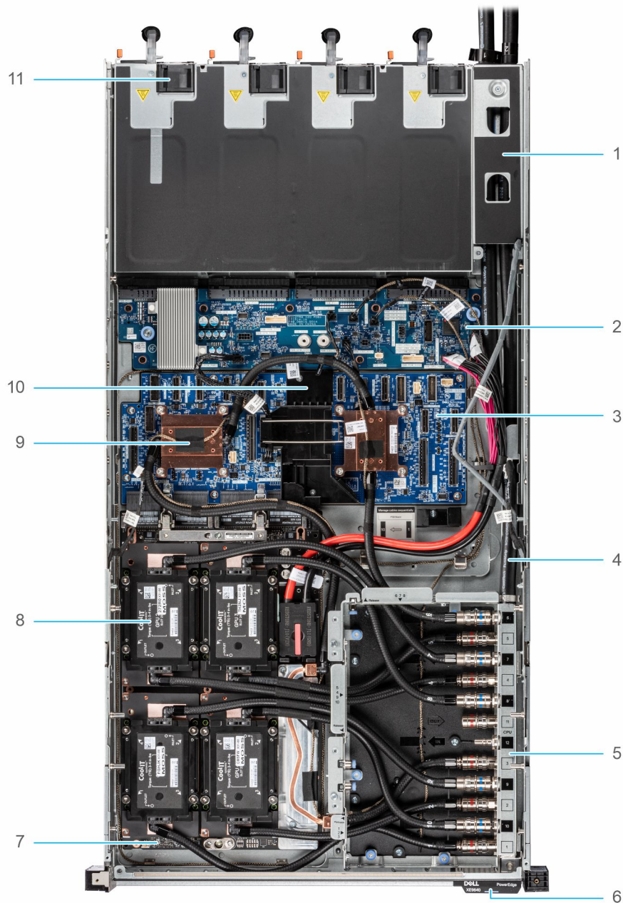
Figure 7. Bottom layer of the XE9640 system with NVIDIA GPUs - inside the system
