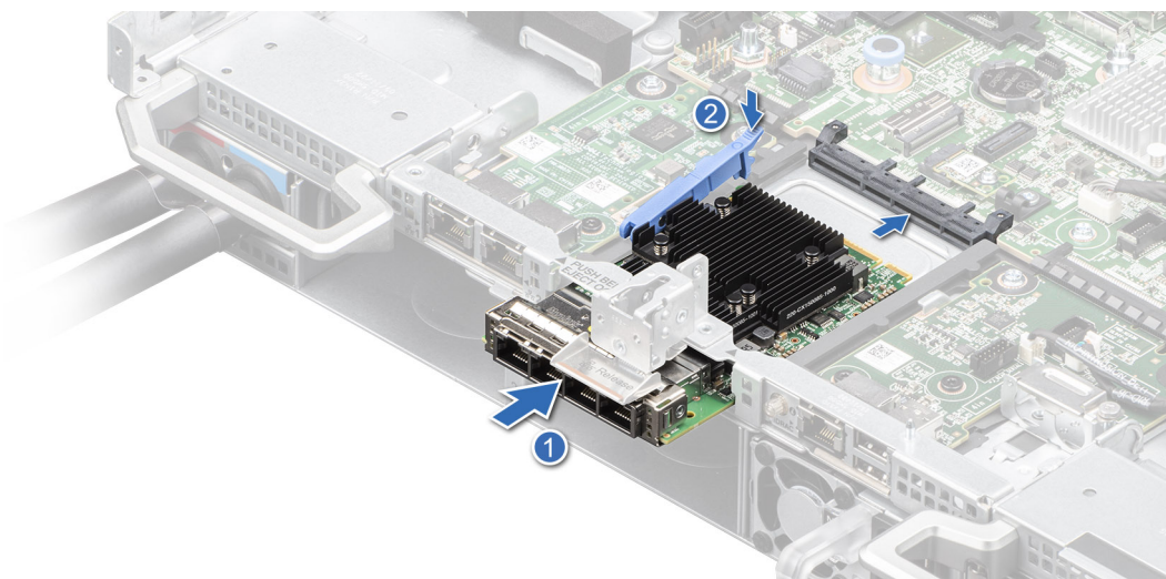
Figure 12. Installing the OCP Card in XE9640
