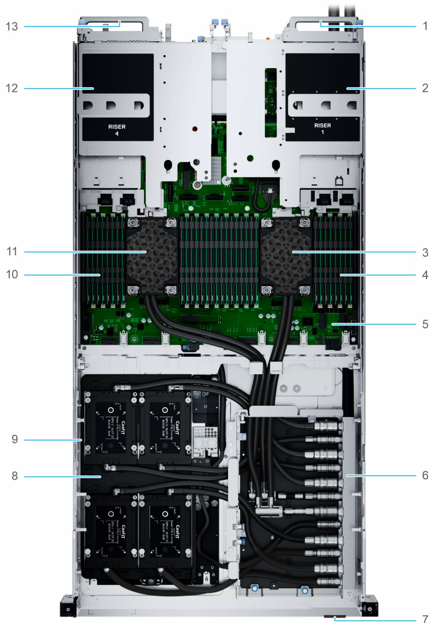
Figure 8. XE9640 with processors and NVIDIA GPUs - inside the system
