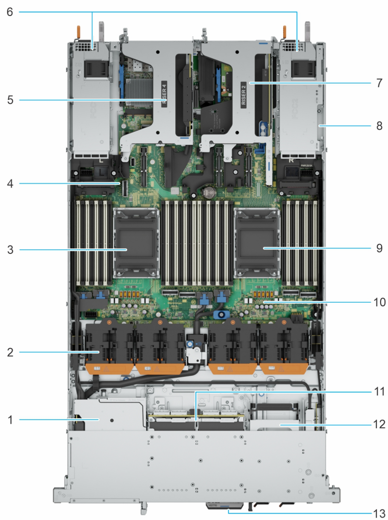
Figure 15. PowerEdge R670 system - inside the system with risers
