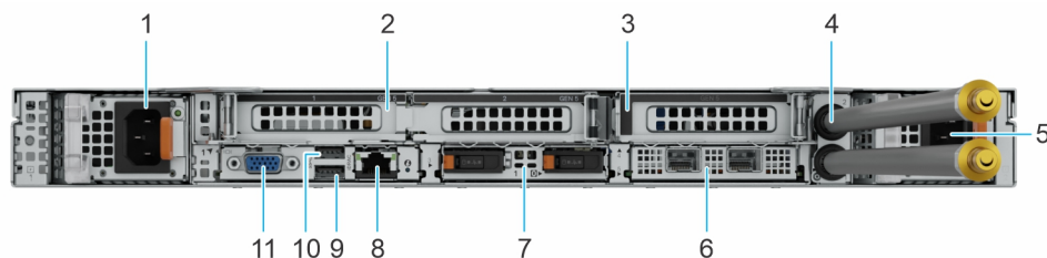
Figure 12. Rear view of the liquid cooling configuration
