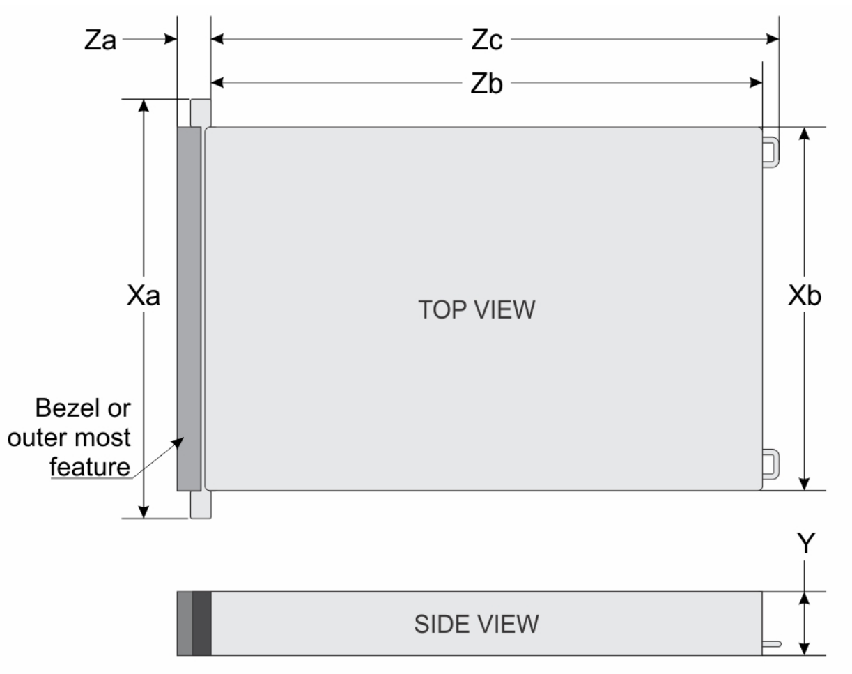
Figure 46. Chassis dimensions
