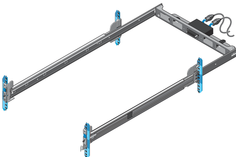
Figure 42. Blind Mate Rails, Rack cabinet members setup
