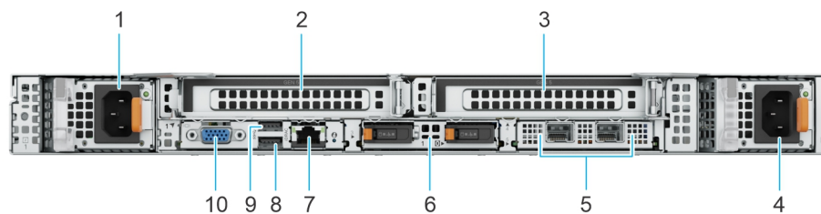
Figure 9. Rear view of the system with rear I/O configuration with riser R2b and R4b
