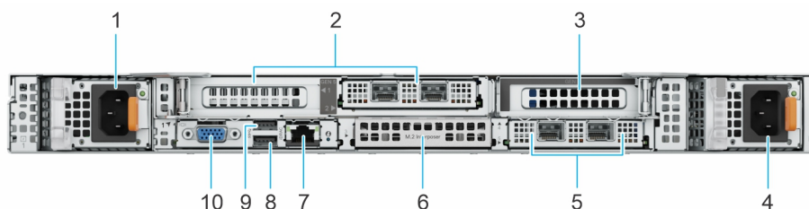
Figure 11. Rear view of the system with rear I/O configuration with riser R2f and R4a and M.2 Interposer board
