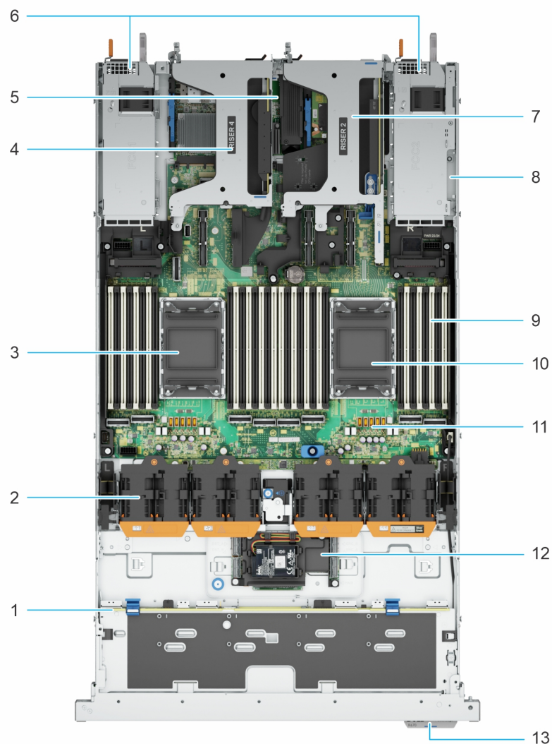
Figure 13. PowerEdge R670 system - inside the system with risers
