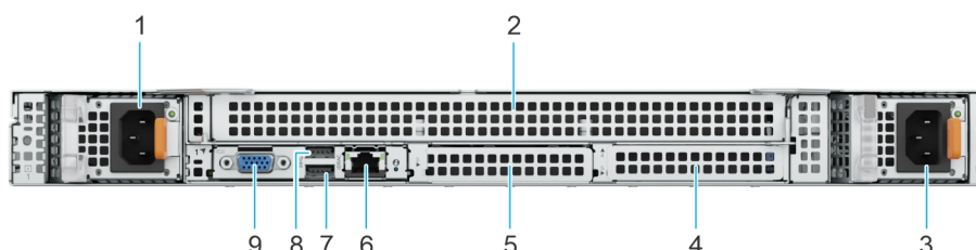
Figure 8. Rear view of the system with front I/O configuration
