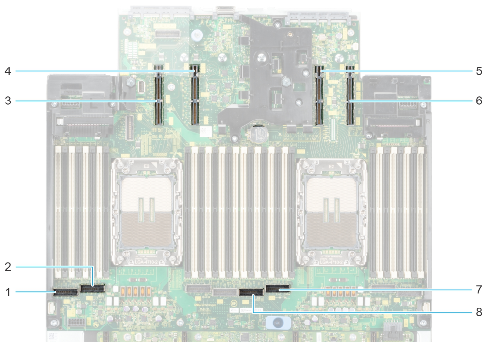
Figure 18. Expansion card riser slot connectors
