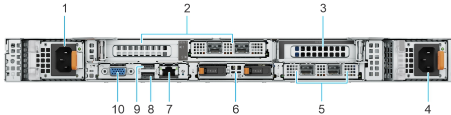
Figure 10. Rear view of the system with rear I/O configuration with riser R2f and R4a
