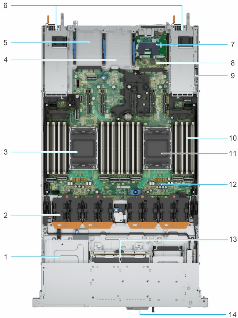
Figure 14. PowerEdge R670 system - inside the system without risers
