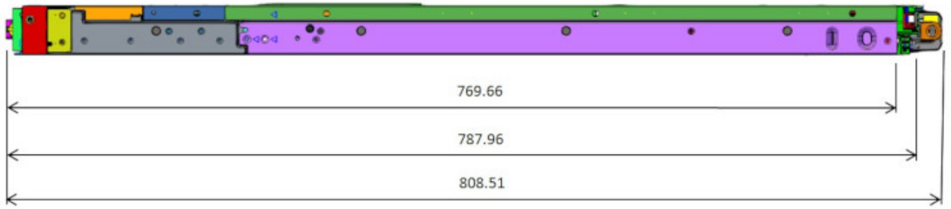
Figure 15. Depth measurements
