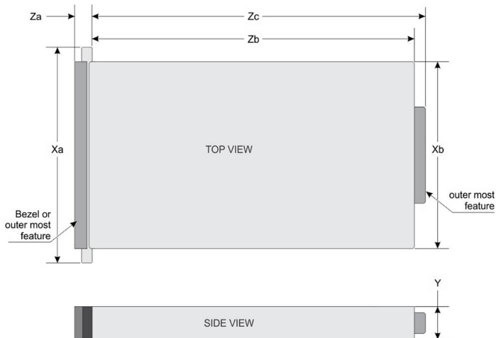
Figure 18. Chassis dimension
