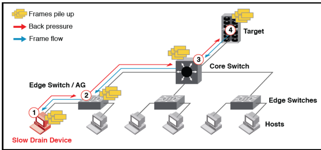
FIGURE 3 Slow-Drain Dataflow
