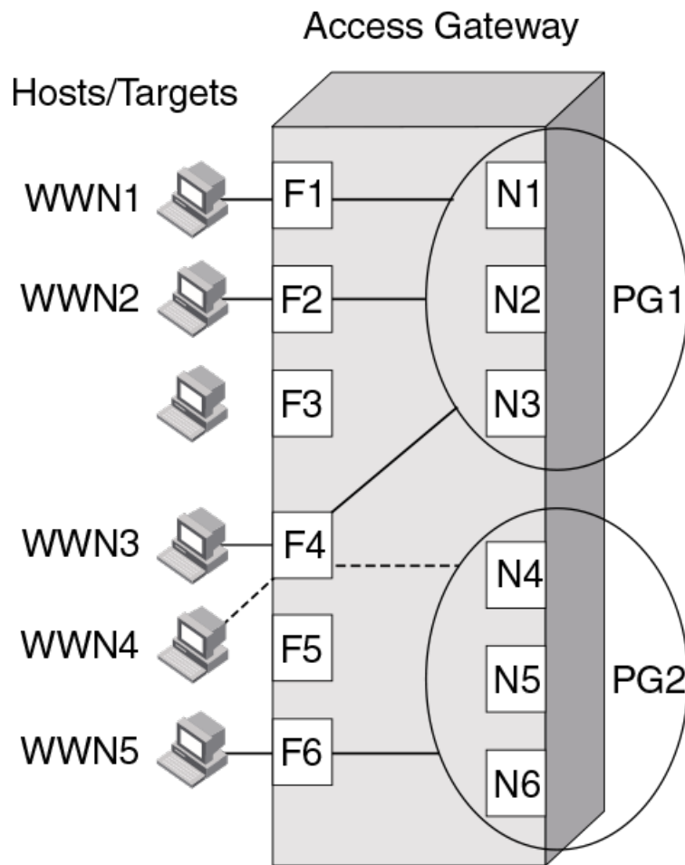
FIGURE 7 Example of device mapping to N_Port groups
