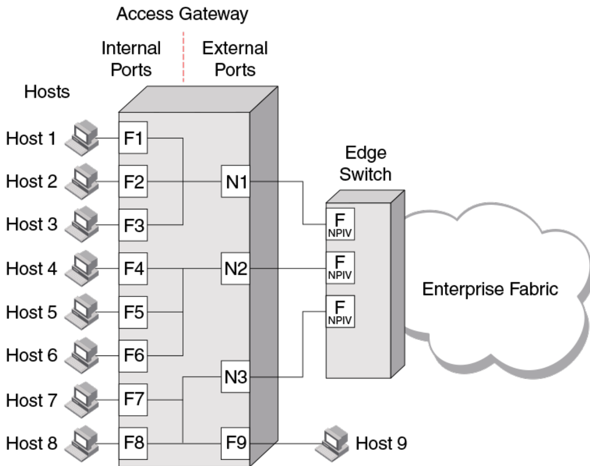
FIGURE 9 Example of adding an external F_Port (F9) on an embedded switch
