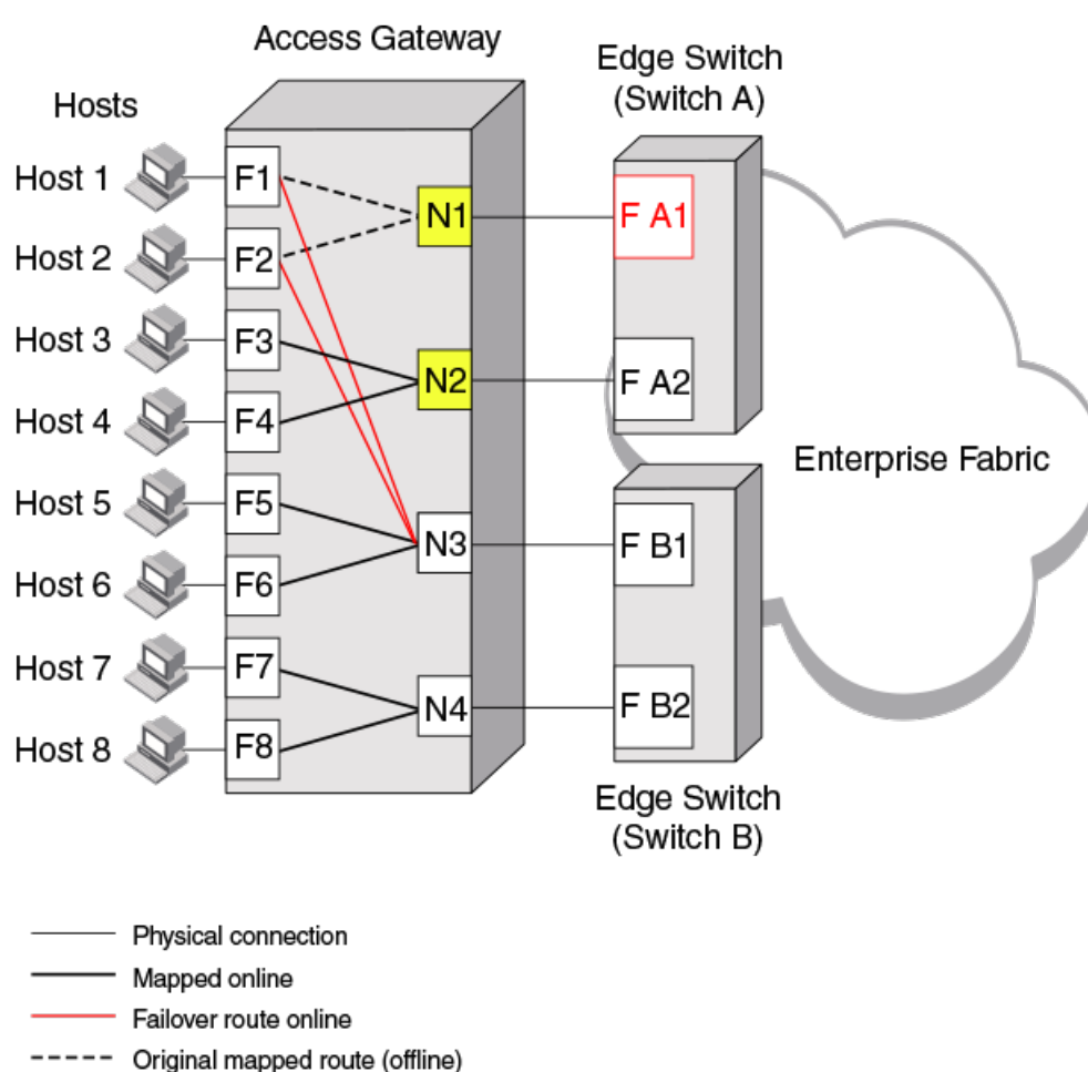
FIGURE 13 Failback behavior
