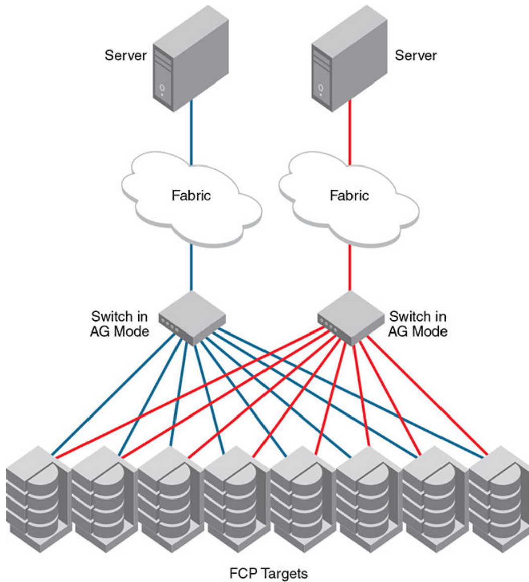
FIGURE 17 Target aggregation
