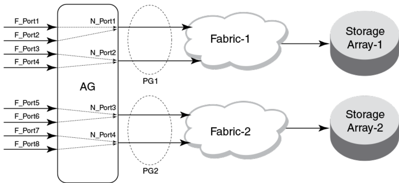
FIGURE 10 Port grouping behavior
