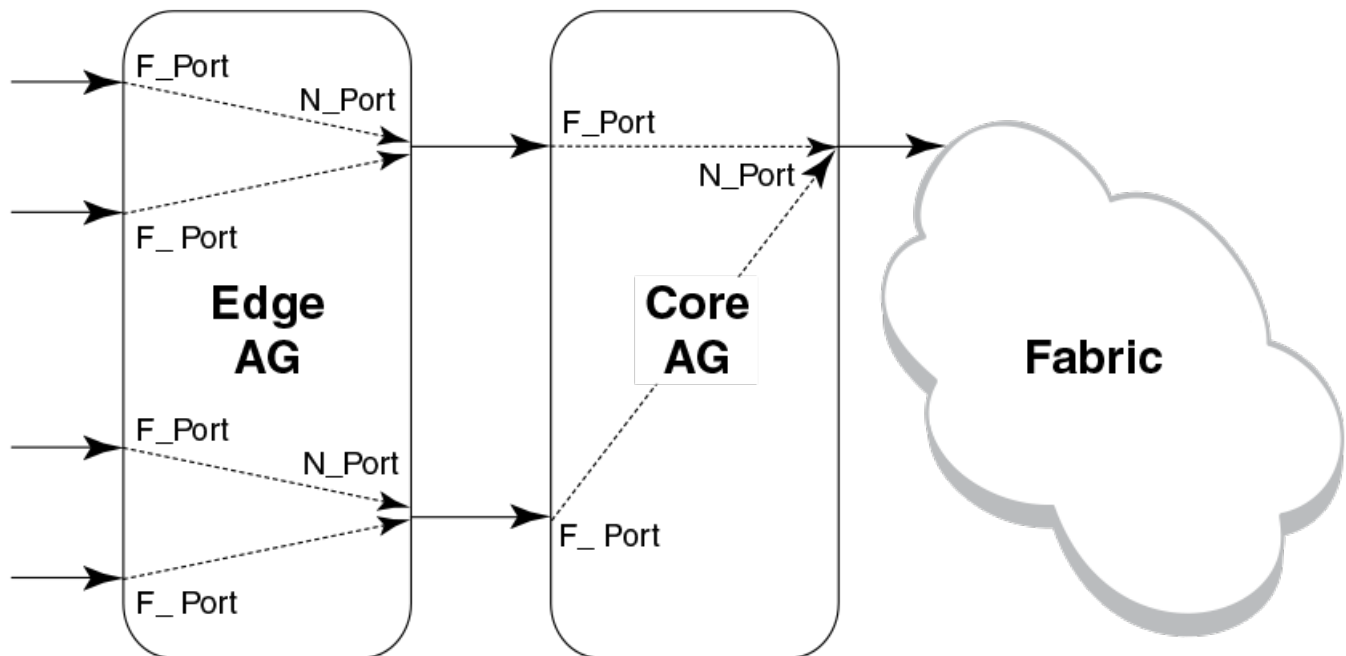
FIGURE 18 Access Gateway cascading
