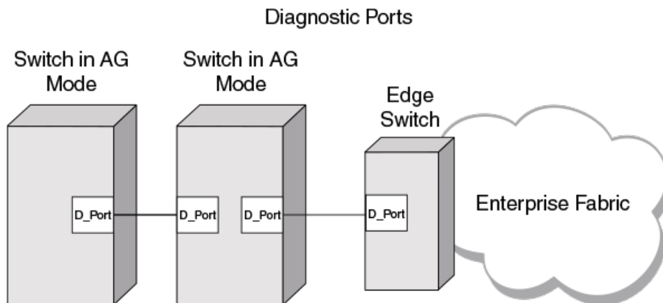
FIGURE 5 Diagnostic Port Configurations
