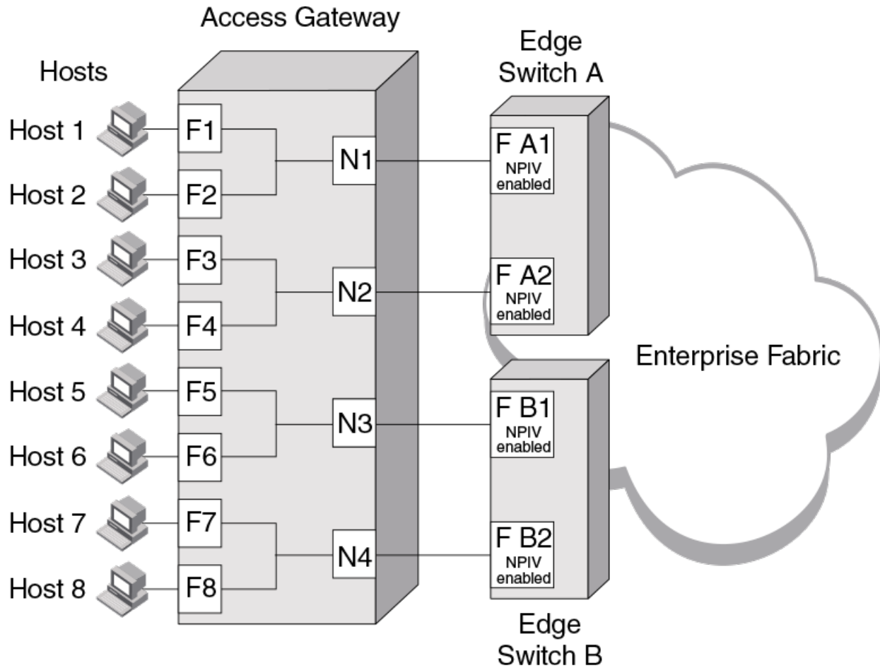
FIGURE 6 Port Mapping Example
