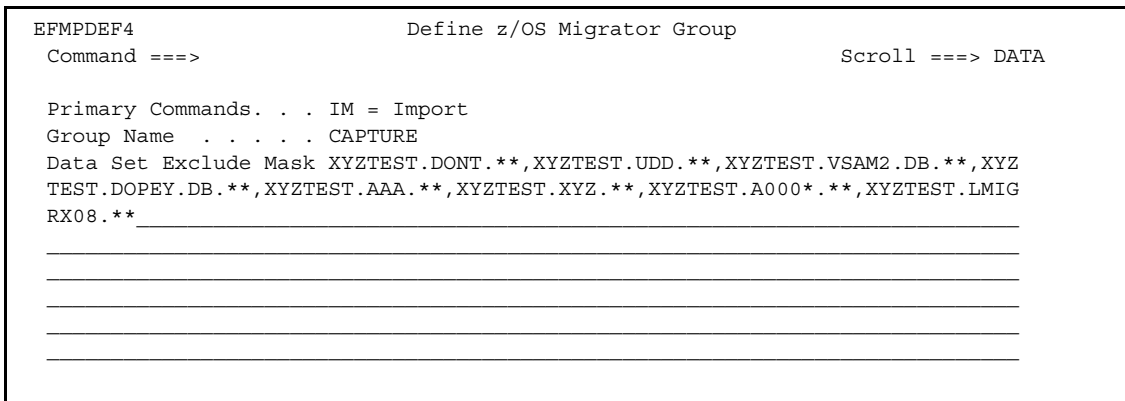
Figure 23 Specify Exclude Masks panel
