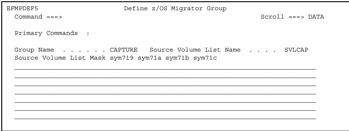
Figure 22 Define Source Volume List panel
