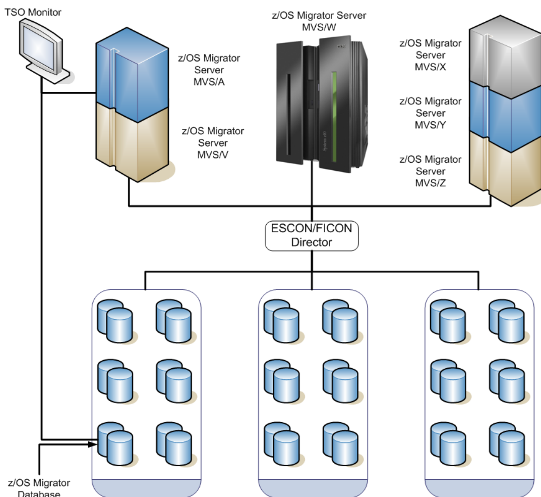
Figure 4 The z/OS Migrator components
