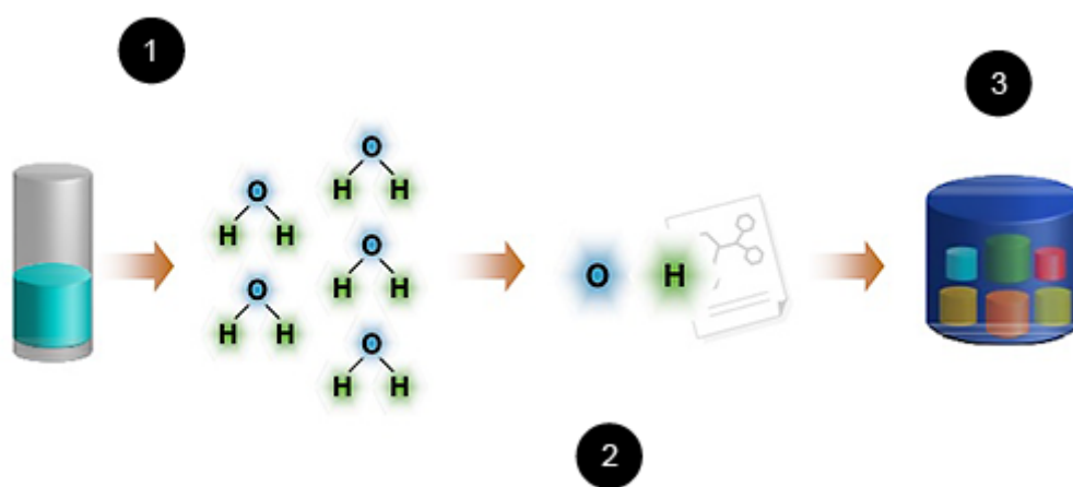
Figure 4. Data deduplication
