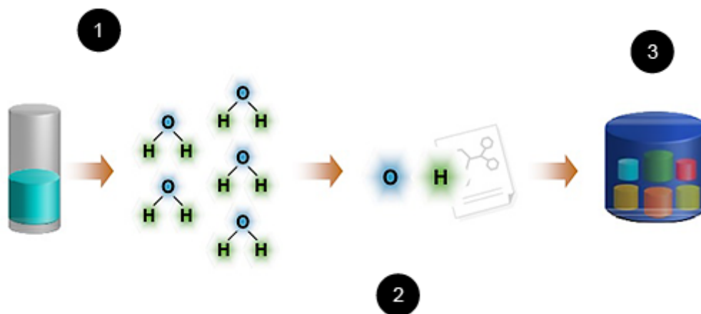
Figure 4. Data deduplication
