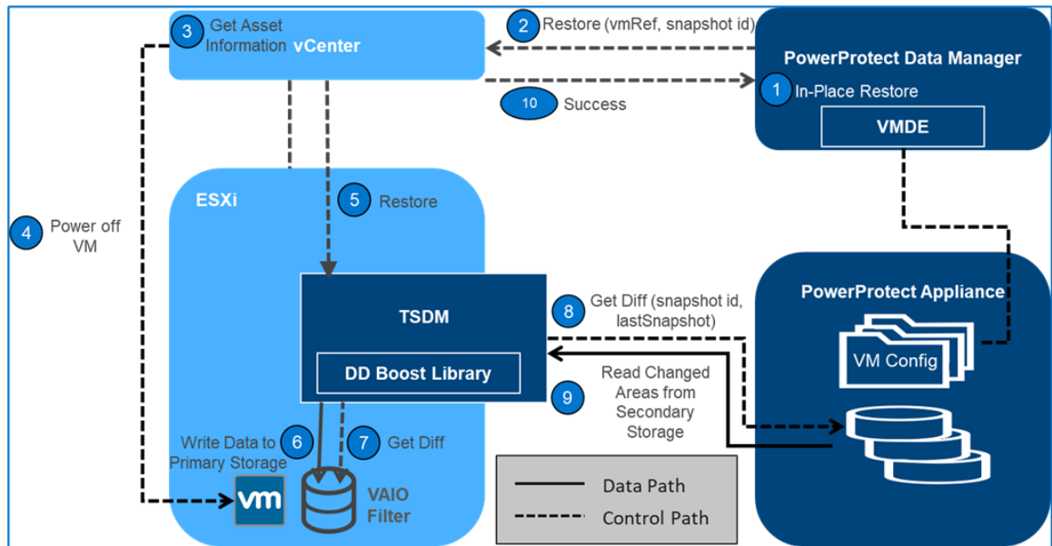
Figure 14. Restoring virtual machines
