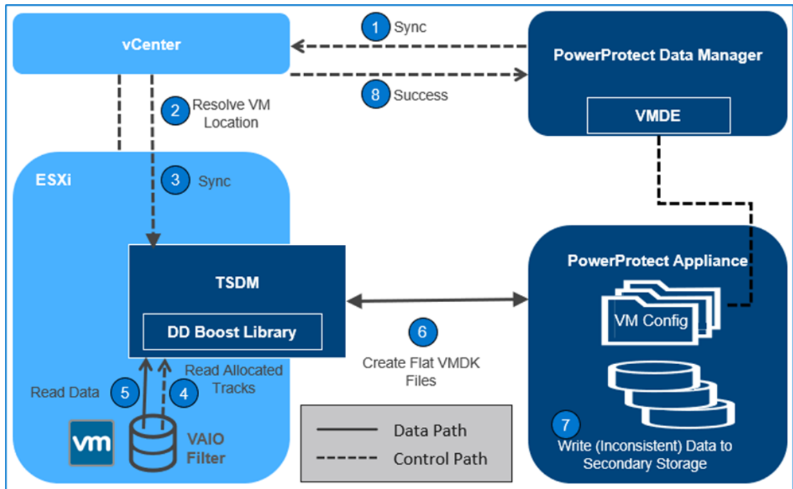
Figure 10. Full sync operation
