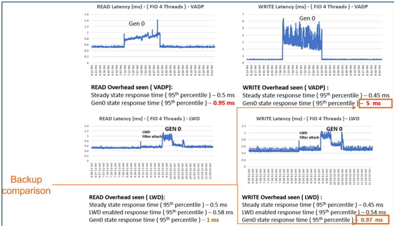
Figure 17. VM latency (read and write) performance comparison
