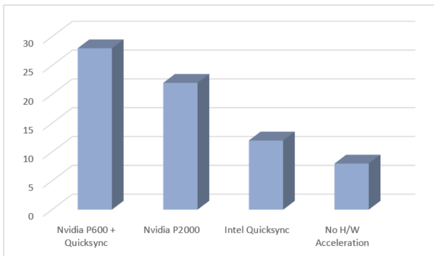
Figure 1. Maximum number of feeds per GPU before frame drops per feed
