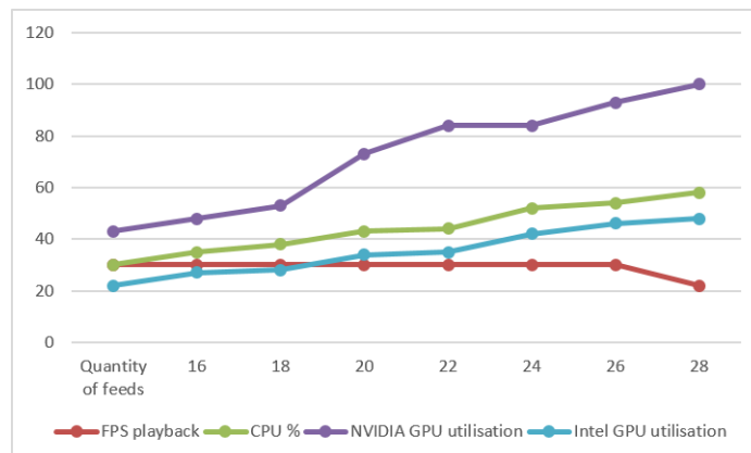
Figure 5. NVIDIA P600 - 1080p feeds at 30 fps
