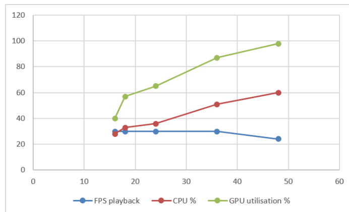
Figure 7. NVIDIA single display - 720p feeds at 30 fps
