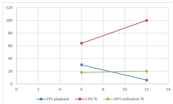
Figure 2. No Hardware Acceleration - 1080p feeds at 30 fps
