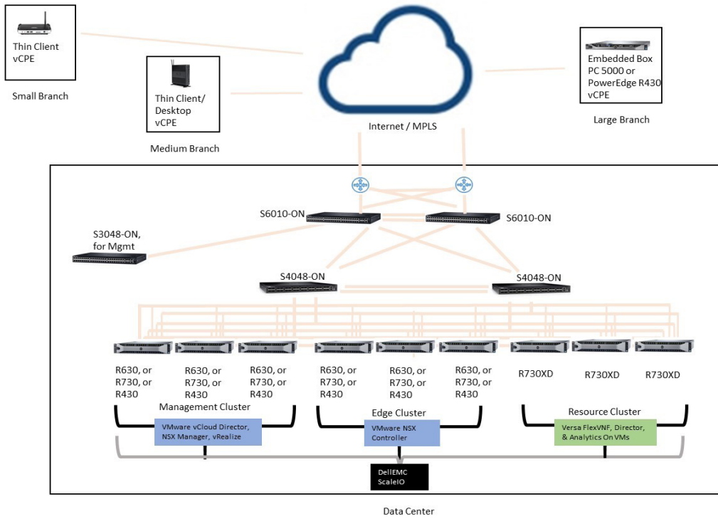
Figure 1: Network diagram for Dell EMC, VMware and Versa solution
