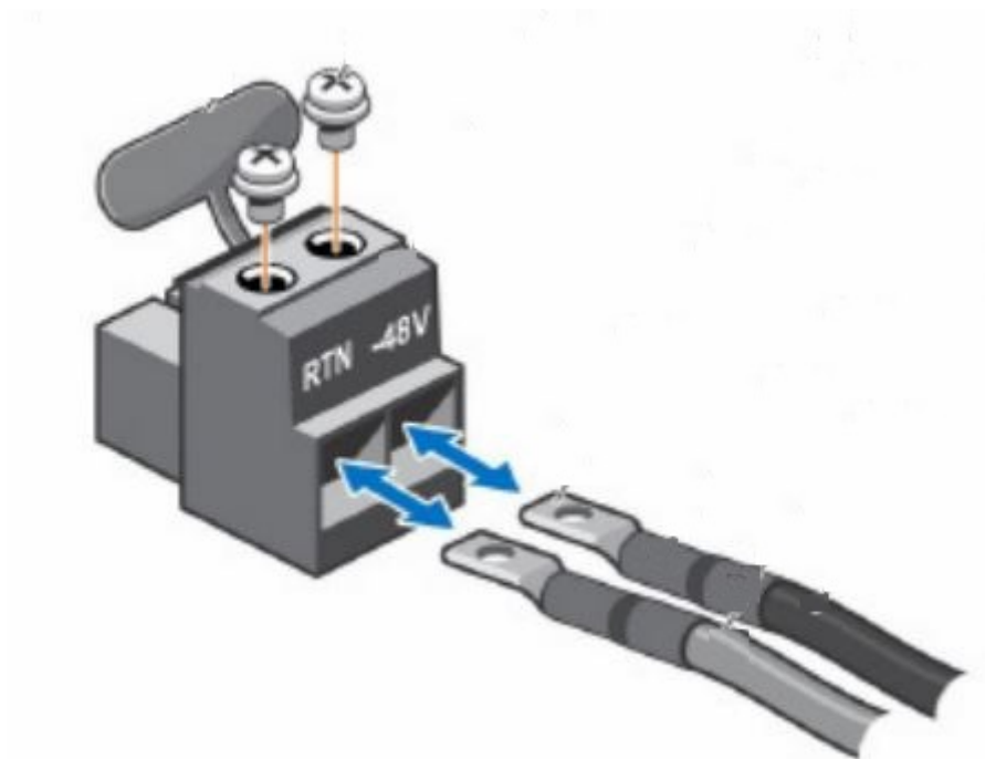
Figure 34. DC PSU power cord
