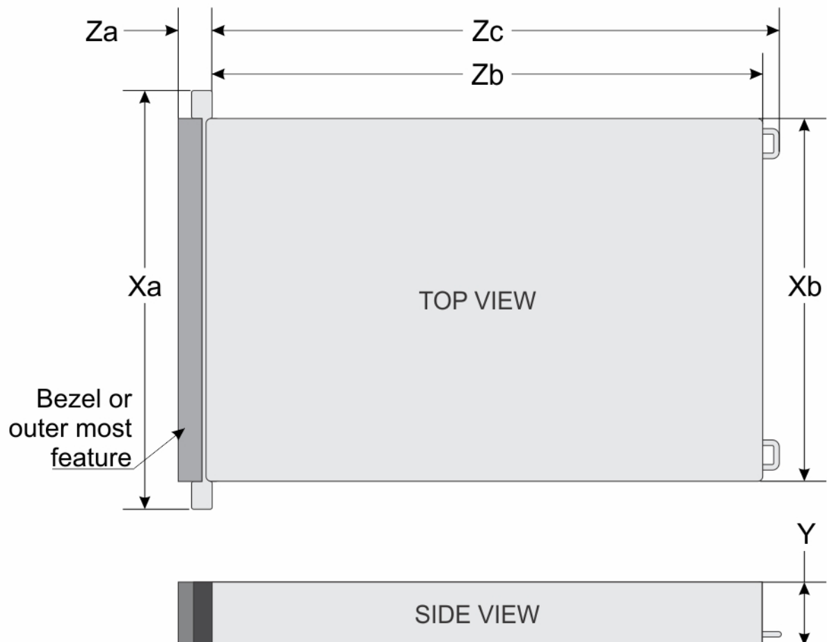
Figure 50. Chassis dimensions
