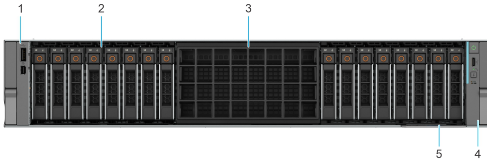
Figure 6. Front view of 16x 2.5-inch SSD system
