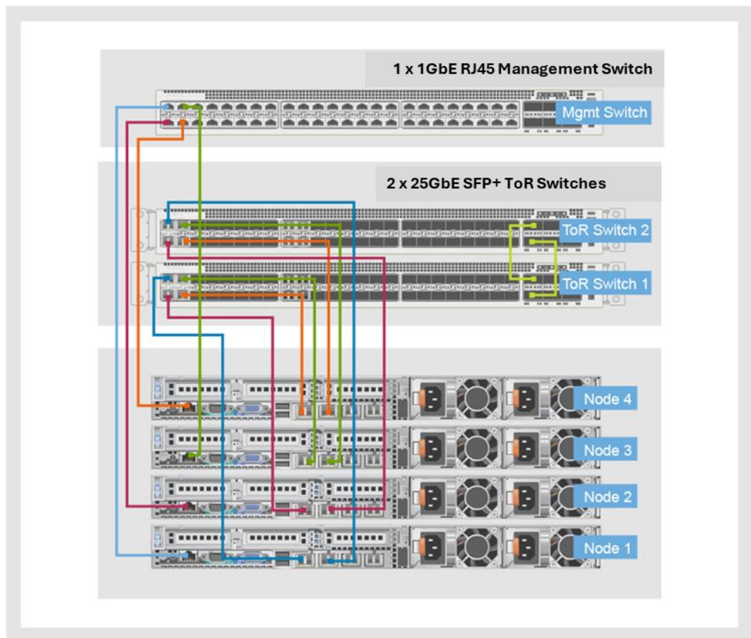
Figure 22. Typical VxRail physical network connectivity for 25 GbE configurations
