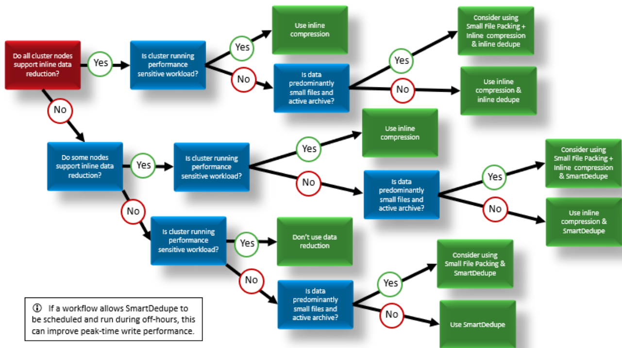
OneFS data reduction and storage efficiency decision tree
