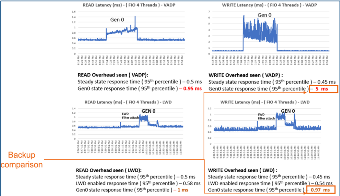
Figure 20. VM latency (read and write) performance comparison
