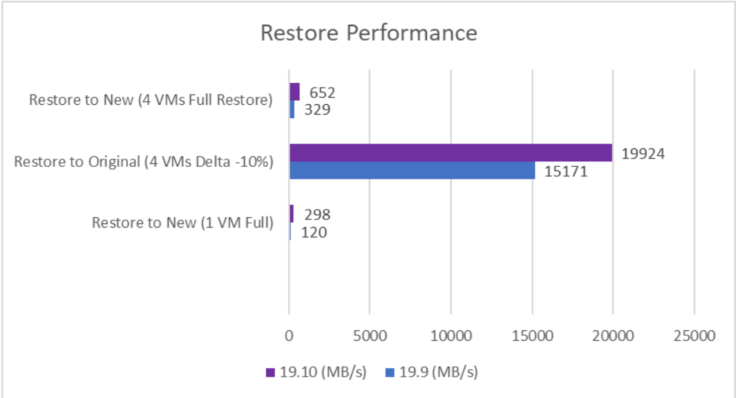
Figure 21. Restore performance comparison
