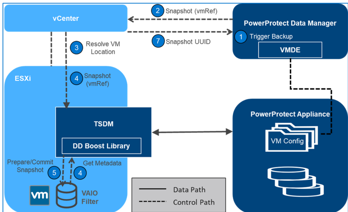
Figure 14. Transparent snapshot creation
