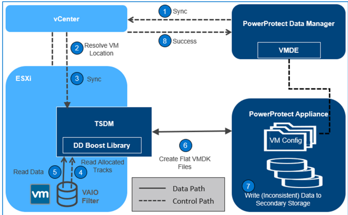
Figure 13. Full sync operation
