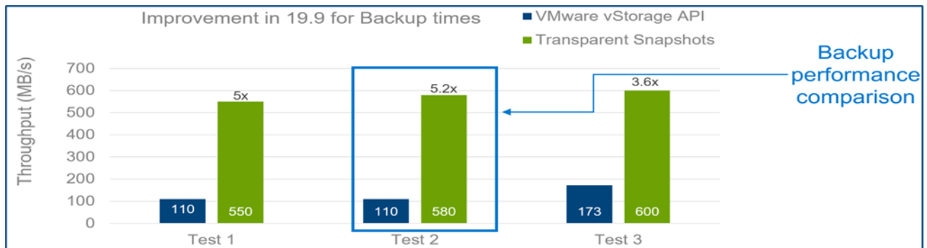
Figure 18. Backup performance comparison
