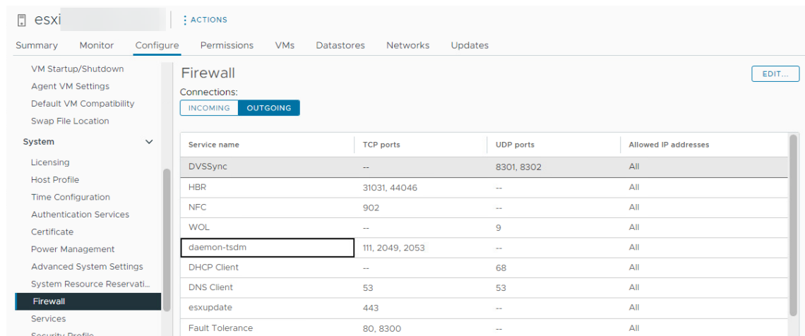
Figure 12. Outline of TSDM required firewall ports
