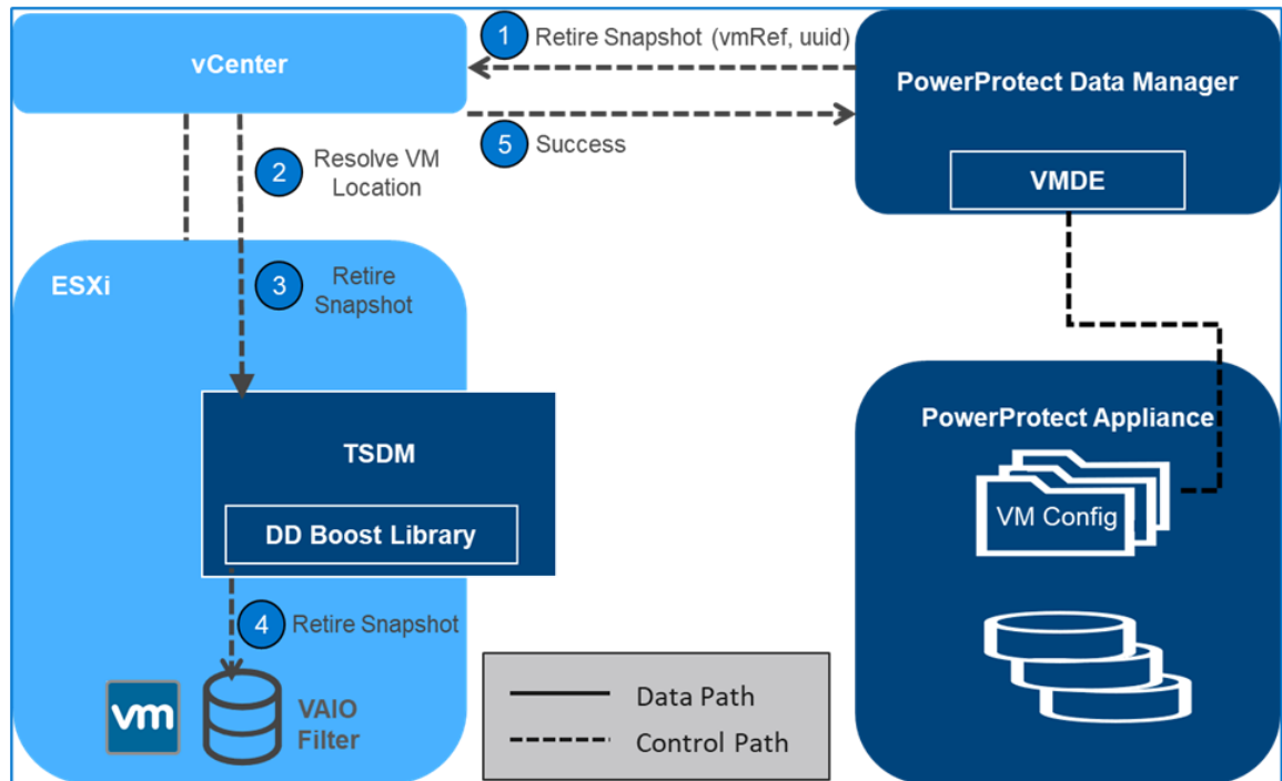
Figure 16. Snapshot retire operation
