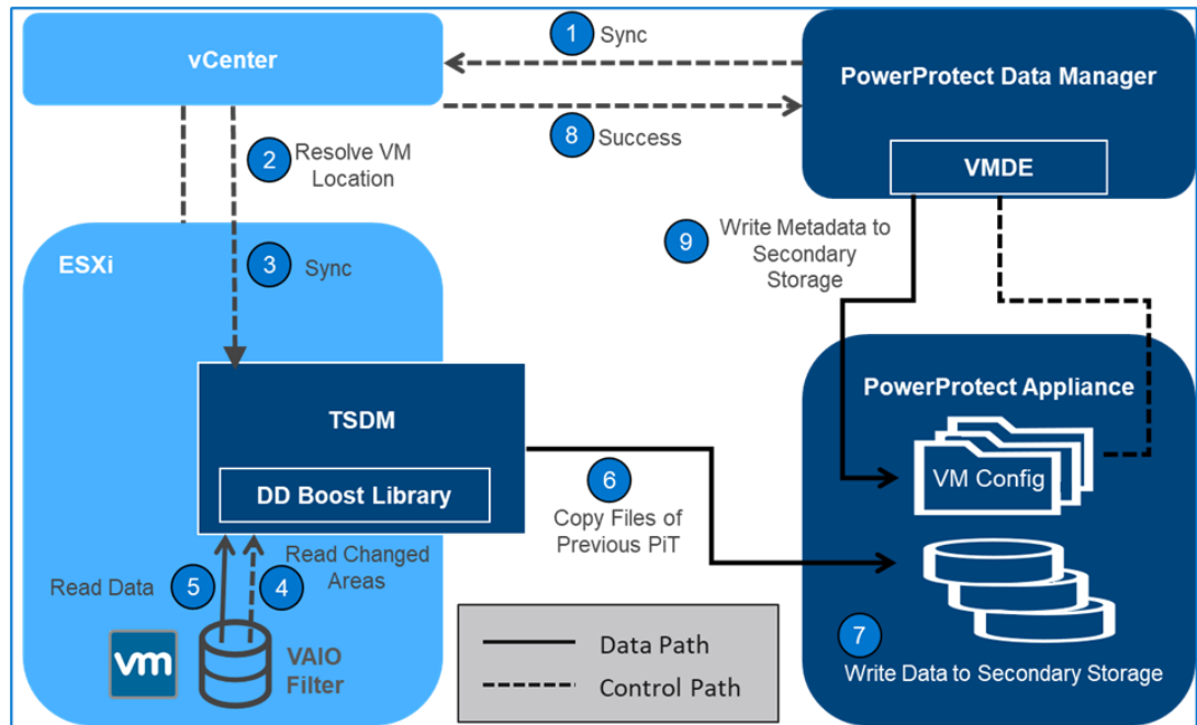
Figure 15. Delta sync operation
