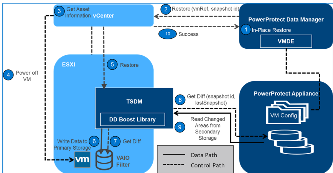
Figure 17. Restoring virtual machines
