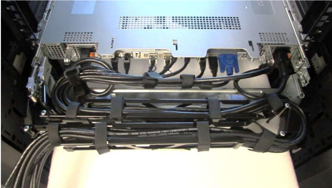
Figure 47. CMA Cabling
