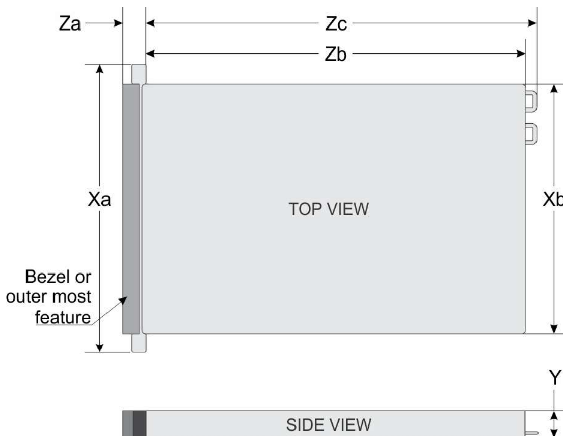
Figure 49. Chassis dimensions
