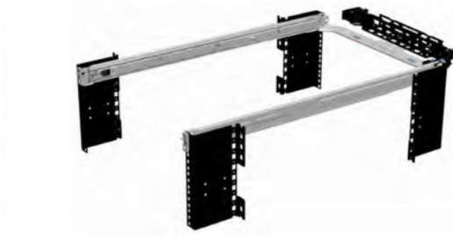
Figure 34. Sliding rails with optional CMA
