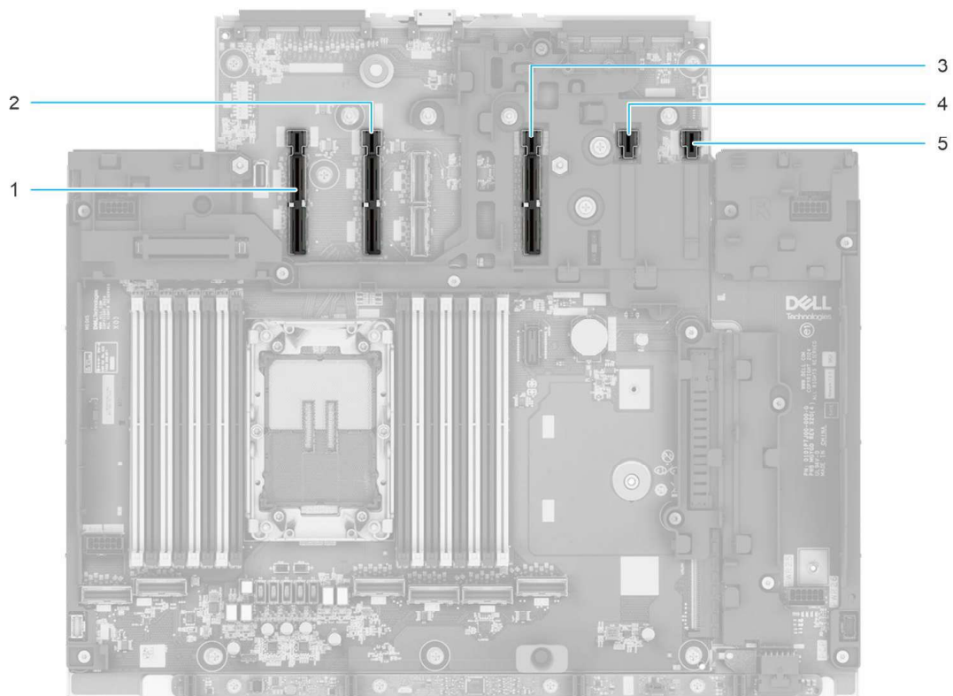
Figure 20. Riser connector location on HPM board
