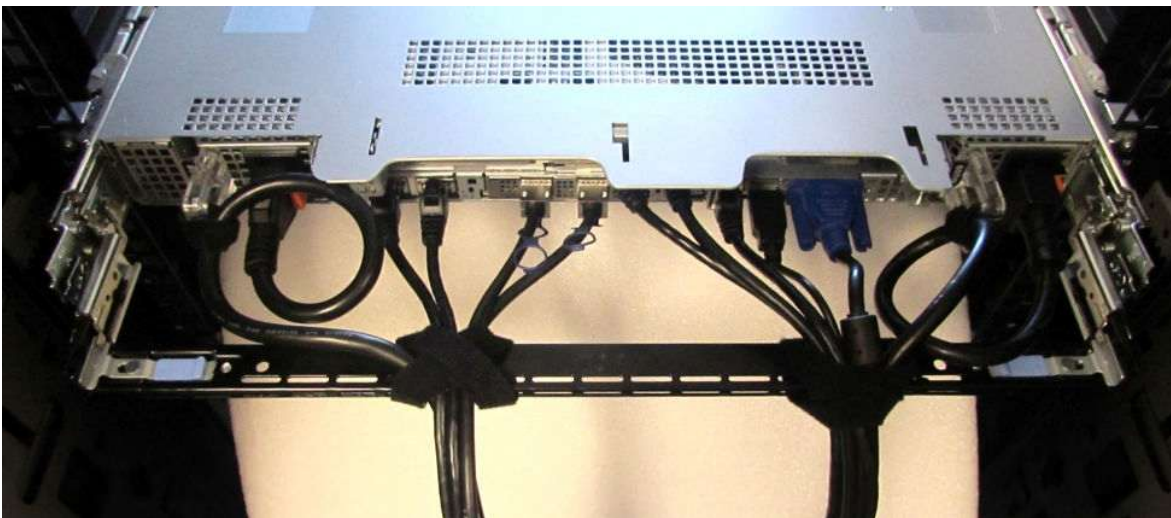
Figure 48. Cabled strain relief bar
